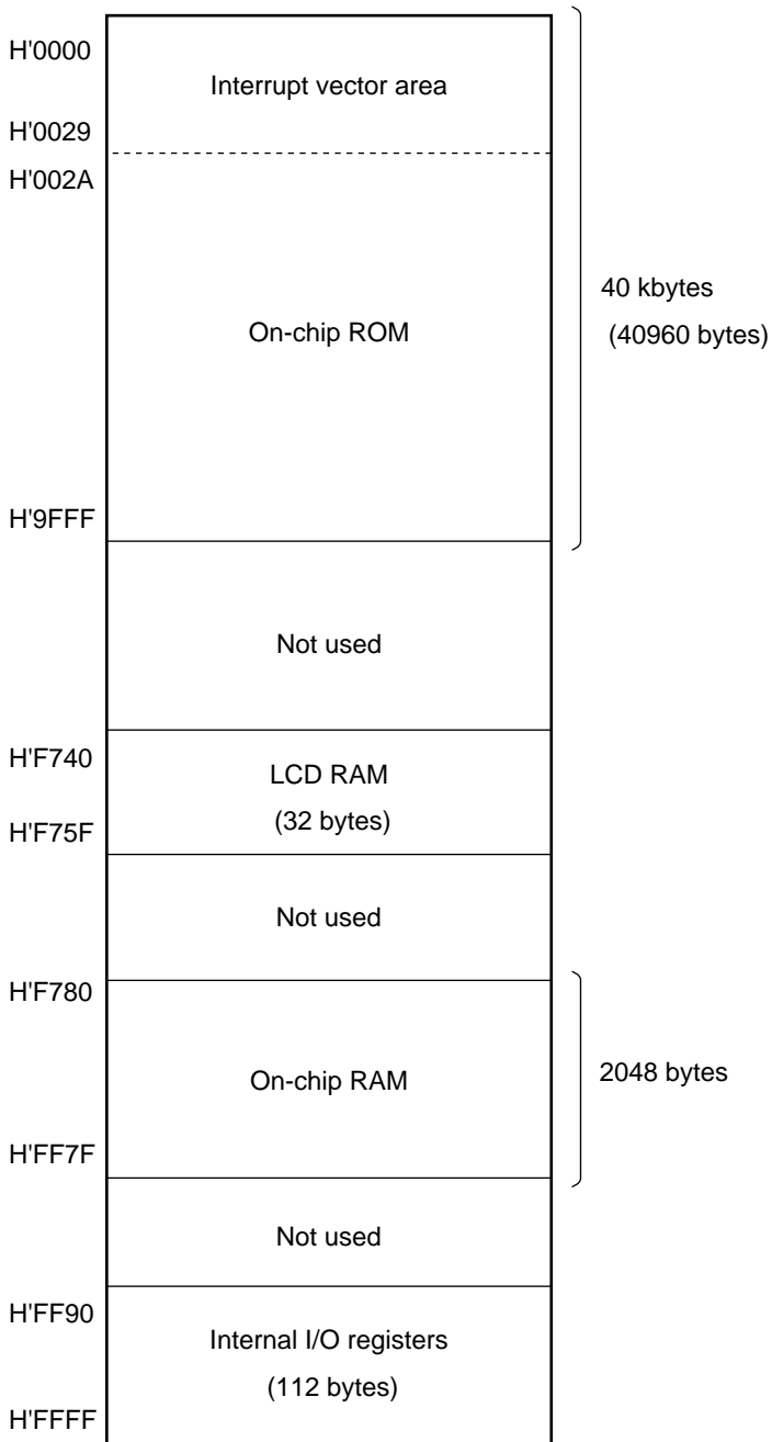
Figure 2-16 (4) H8/3885 and H8/3845 Memory Map
