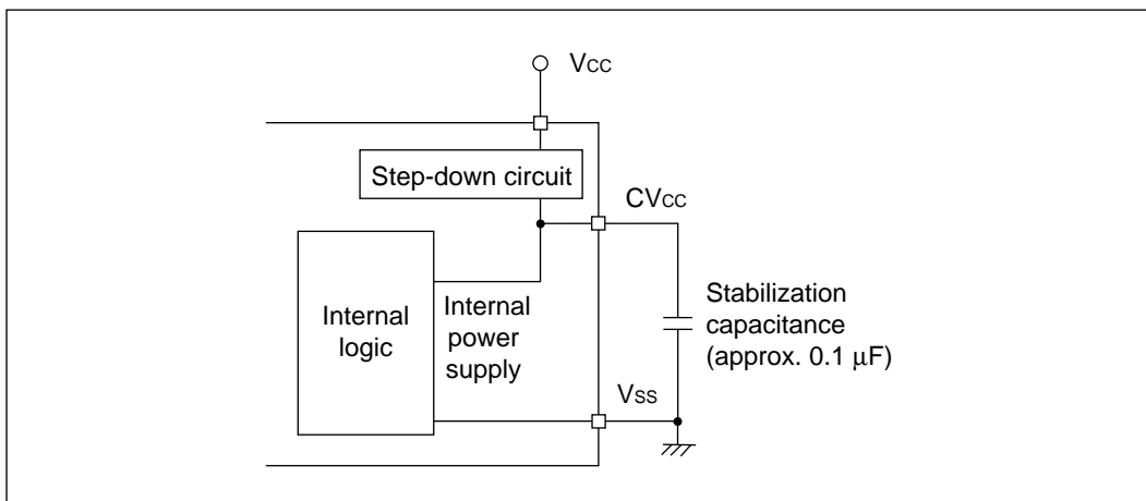
Figure 14-1 Power Supply Connection when Internal Step-Down Circuit Is Used
