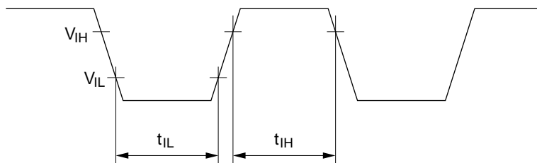
Figure 15-3 Input Timing
