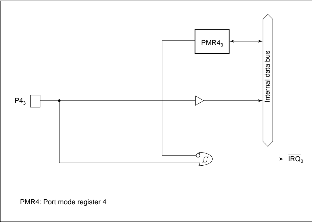
Figure C.4 (a) Port 4 Block Diagram (Pin P4_3 )
