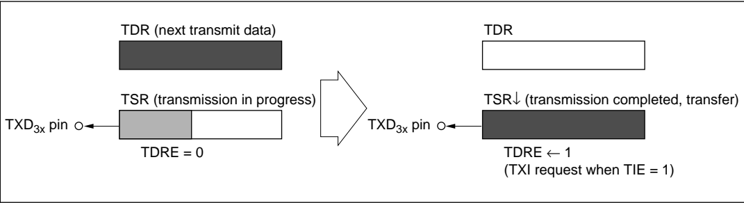
Figure 10-7 (b) TDRE Setting and TXI Interrupt
