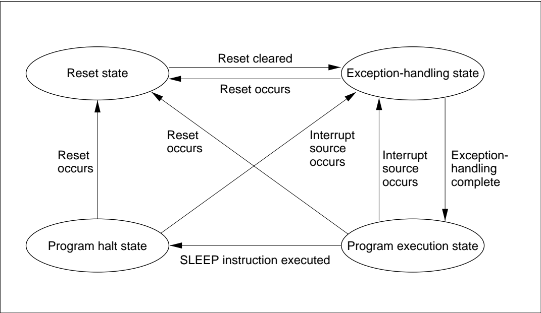
Figure 2-15 State Transitions
