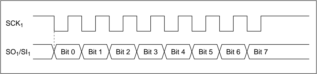
Figure 10-2 Transfer Format
