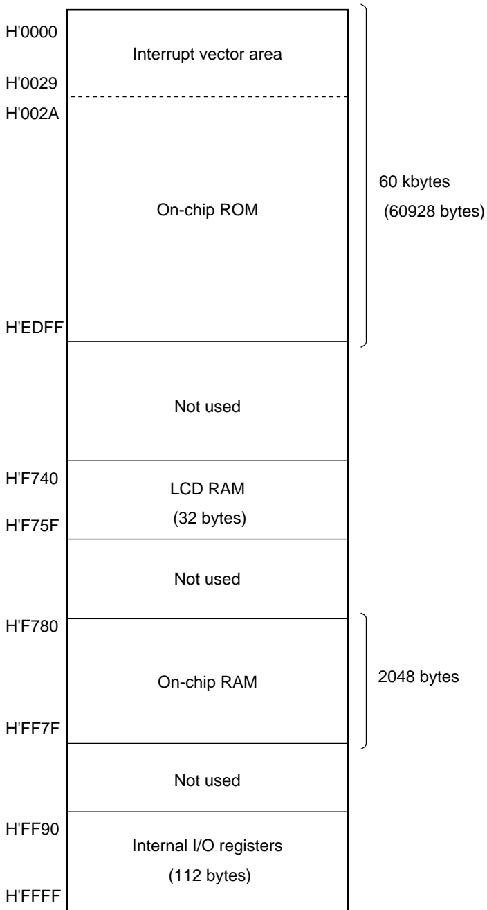
Figure 2-16 (6) H8/3887 and H8/3847 Memory Map
