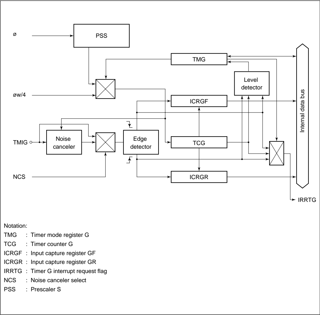
Figure 9-7 Block Diagram of Timer G
