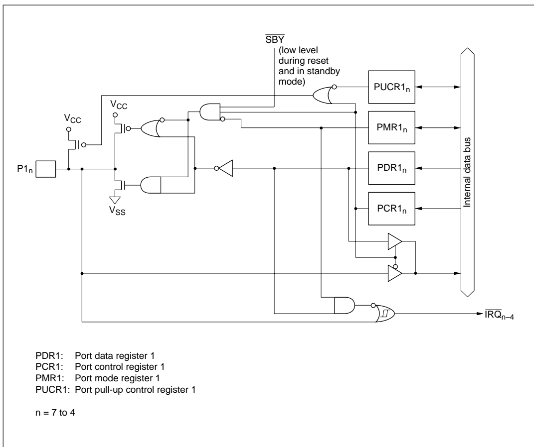
Figure C-1 (a) Port 1 Block Diagram (Pins P1_7 to P1_4 )
