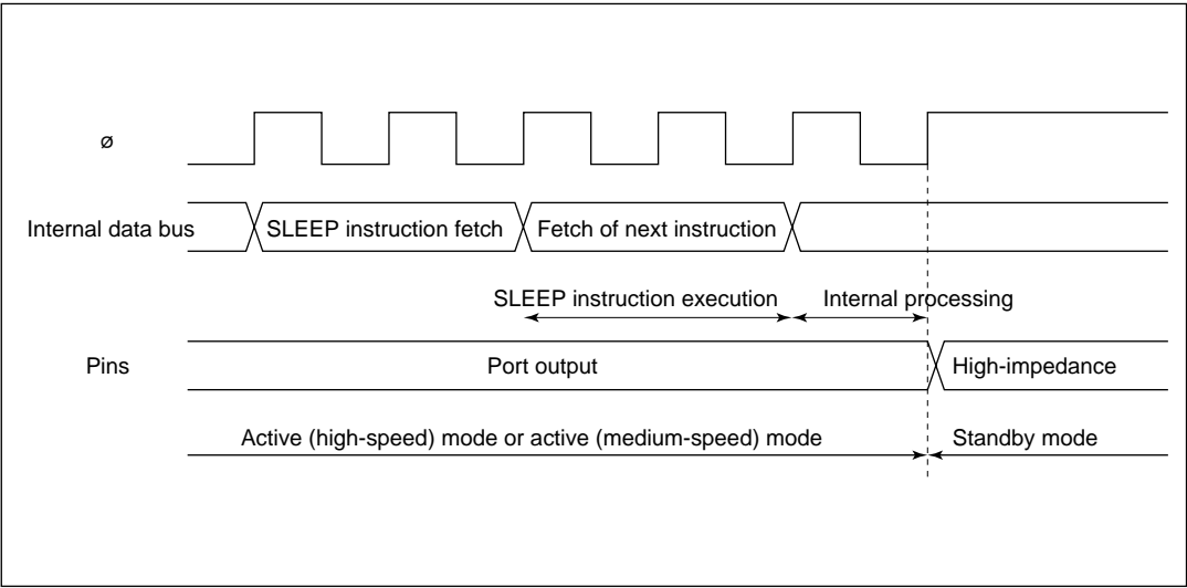
Figure 5-2 Standby Mode Transition and Pin States
