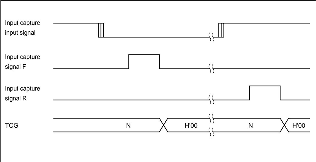
Figure 9-13 TCG Clear Timing
