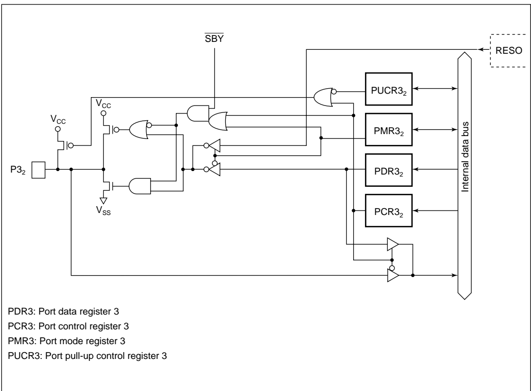
Figure C.3 (e) Port 3 Block Diagram (Pin P3 2 )
