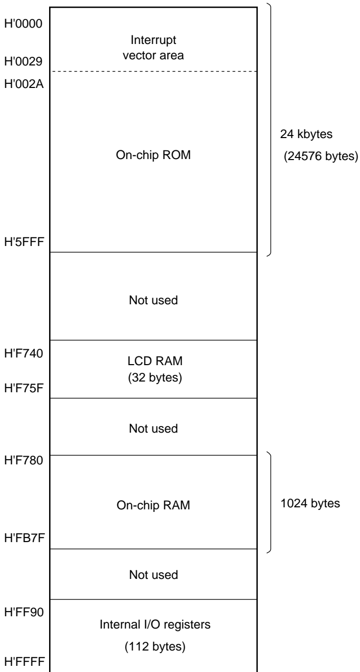
Figure 2-16 (2) H8/3883 and H8/3843 Memory Map
