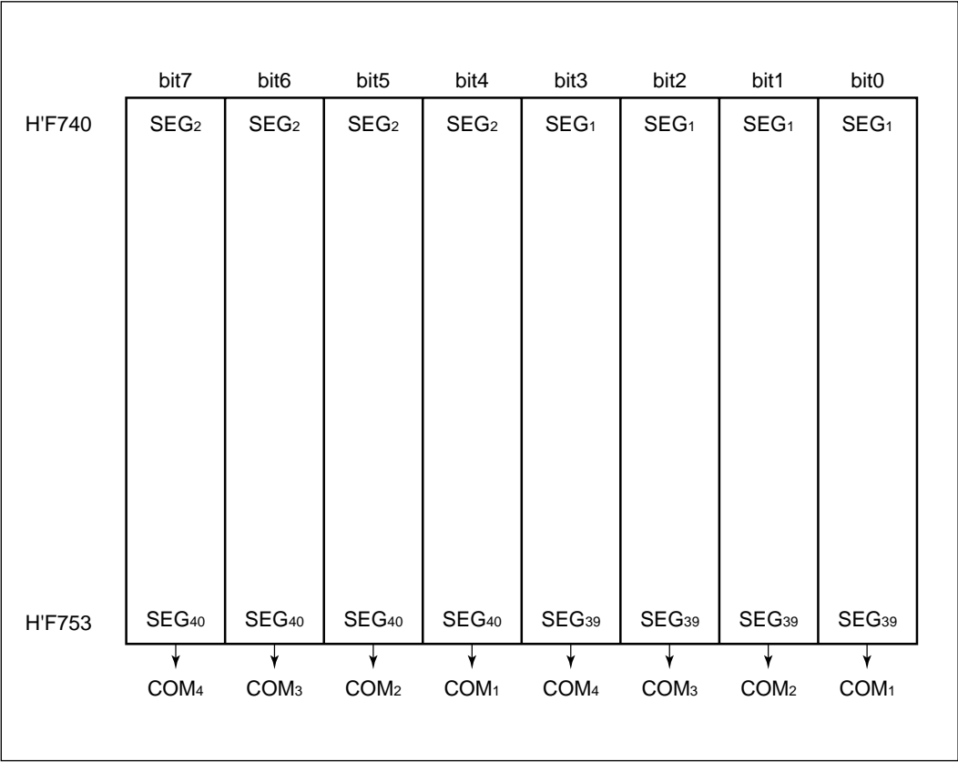
Figure 13-5 LCD RAM Map with Segments Not Externally Expanded (1/4 Duty)
