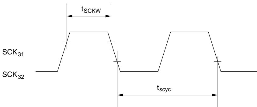
Figure 15-6 SCK3 Input Clock Timing
