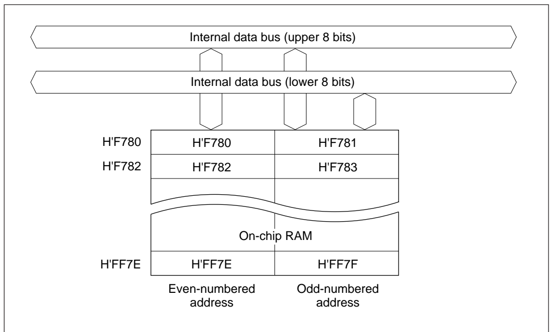
Figure 7-1 RAM Block Diagram (H8/3884, H8/3844)
