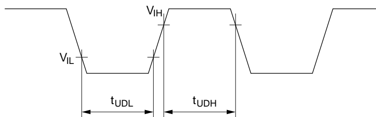
Figure 15-4 UD Pin Minimum Modulation Width Timing
