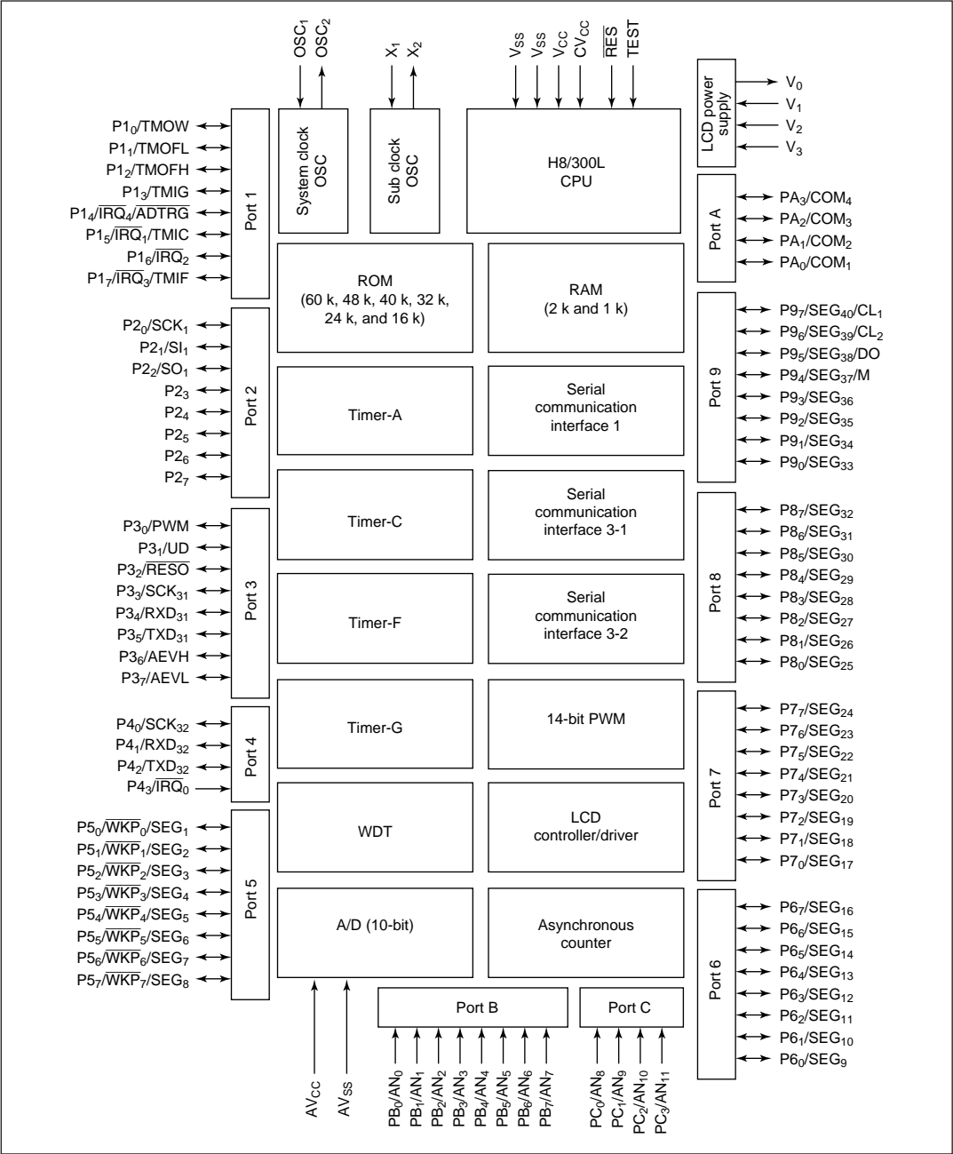
Figure 1-1 Block Diagram
