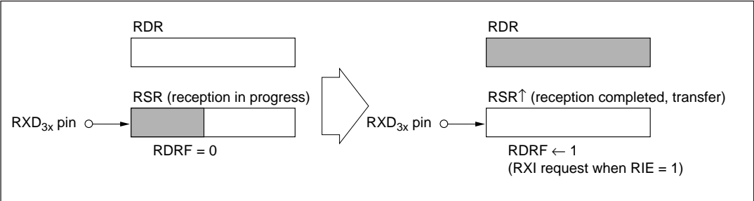
Figure 10-2 (a) RDRF Setting and RXI Interrupt
