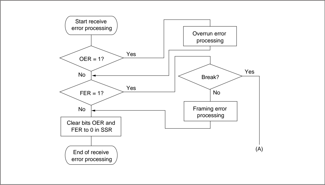
Figure 10-19 Example of Multiprocessor Data Reception Flowchart (cont)
