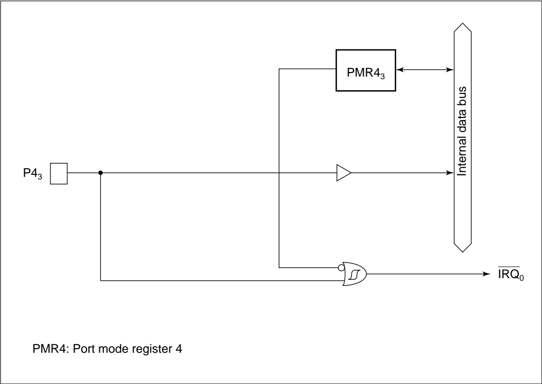
Figure C.3 (a) Port 4 Block Diagram (Pin P4 3 )
