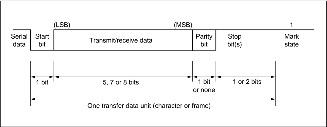
Figure 10-3 Data Format in Asynchronous Communication
