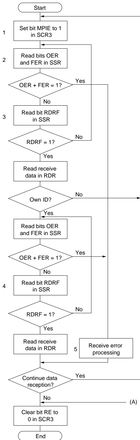
Figure 10-19 Example of Multiprocessor Data Reception Flowchart
