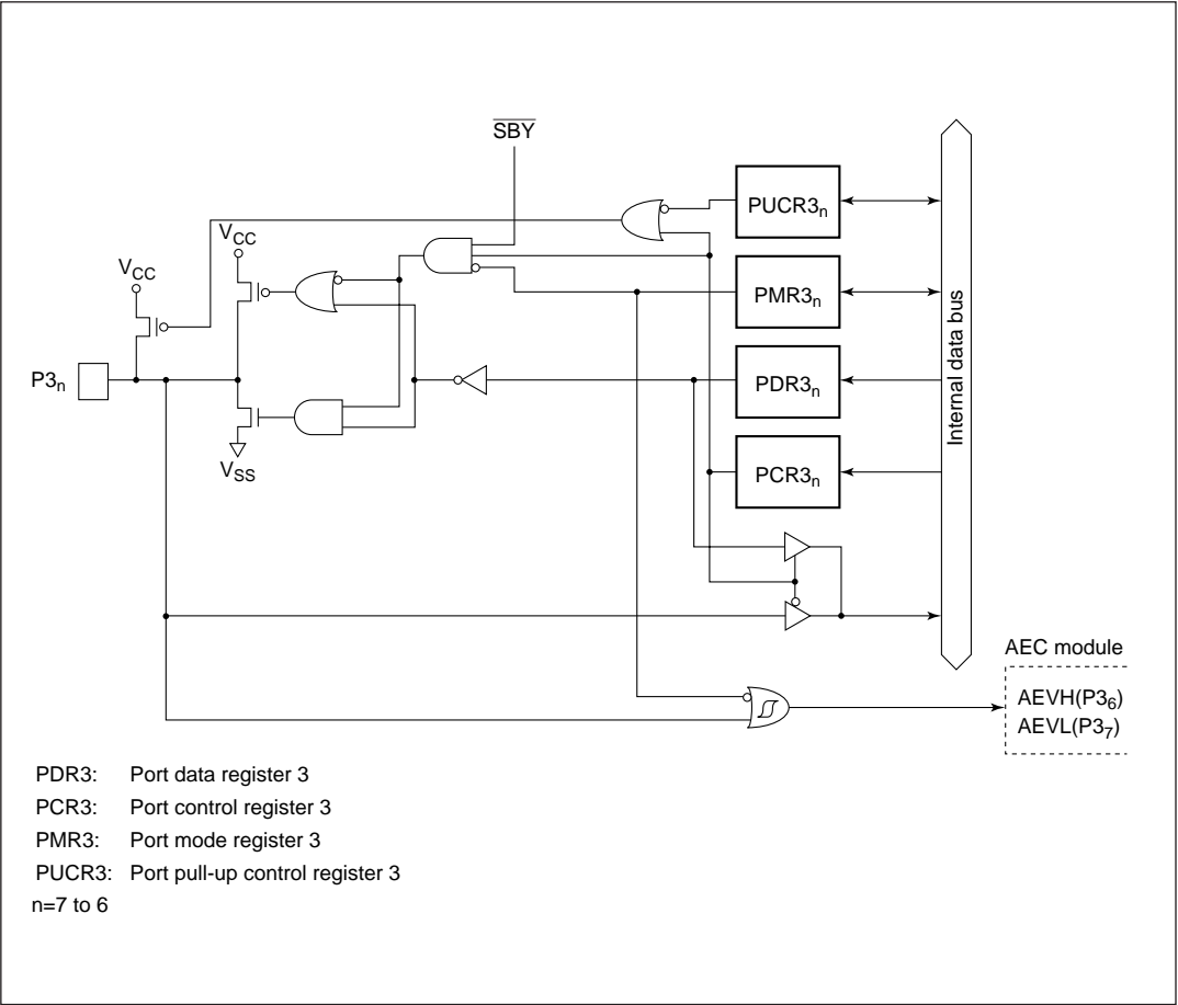
Figure C-2 (a) Port 3 Block Diagram (Pin P3 7 to P3 6 )
