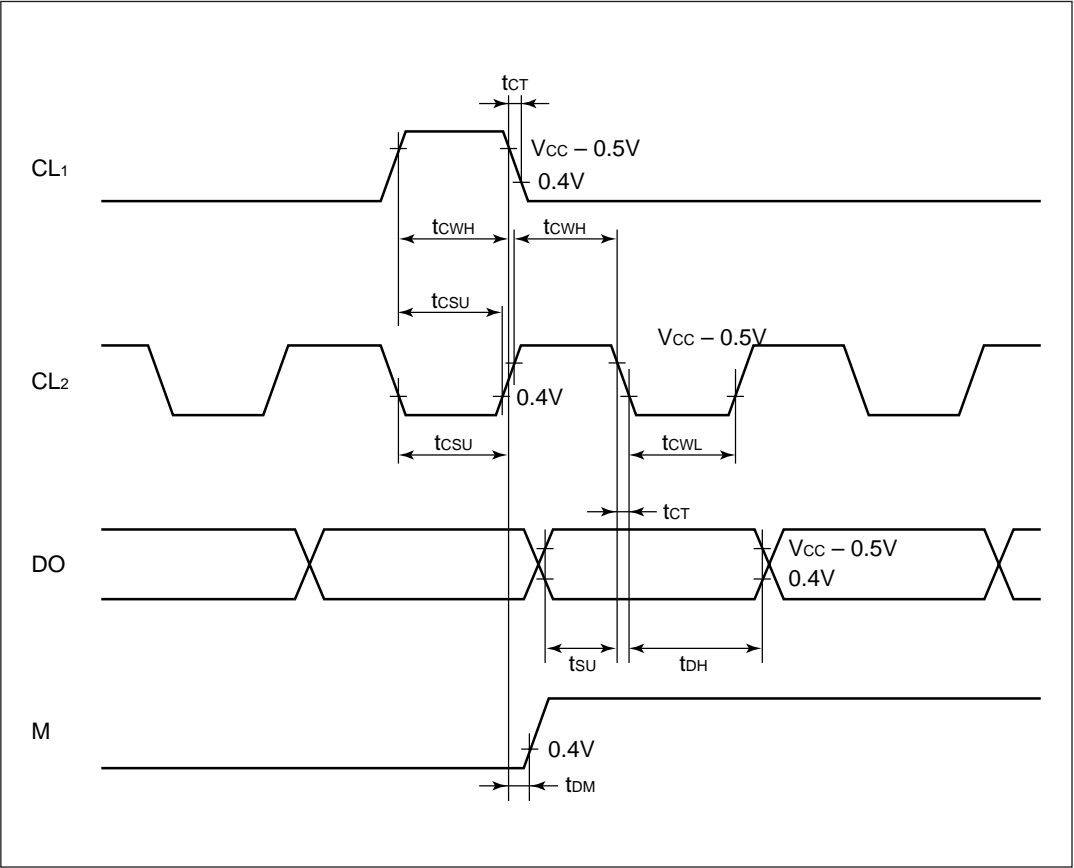
Figure 15-7 Segment Expansion Signal Timing
