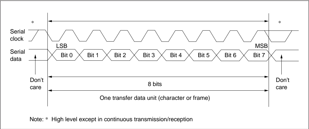
Figure 10-10 Data Format in Synchronous Communication
