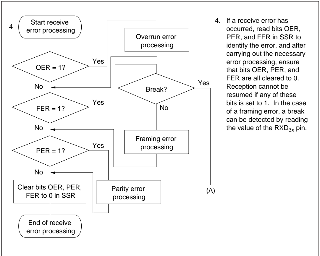
Figure 10-8 Example of Data Reception Flowchart (Asynchronous Mode) (cont)
