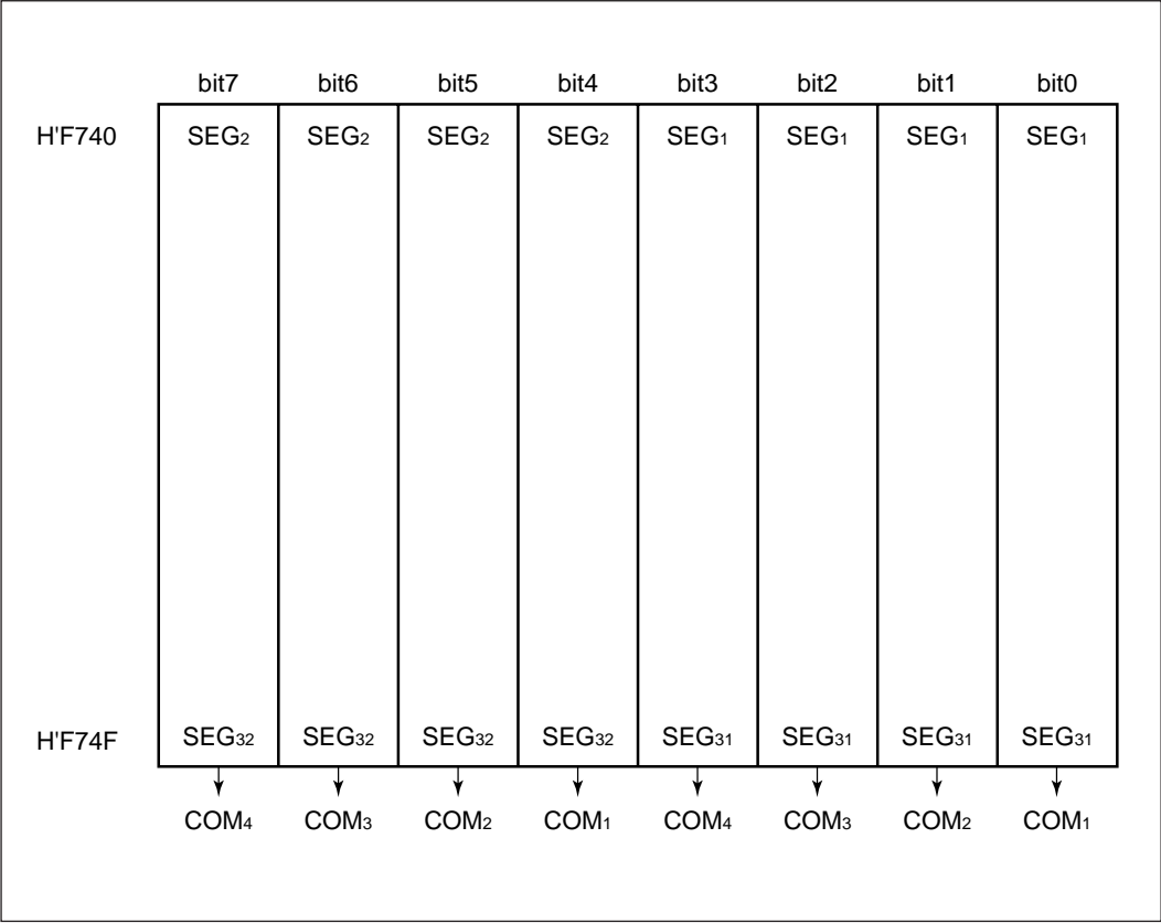
Figure 13-5 LCD RAM Map when Not Using Segment External Expansion (1/4 Duty)
