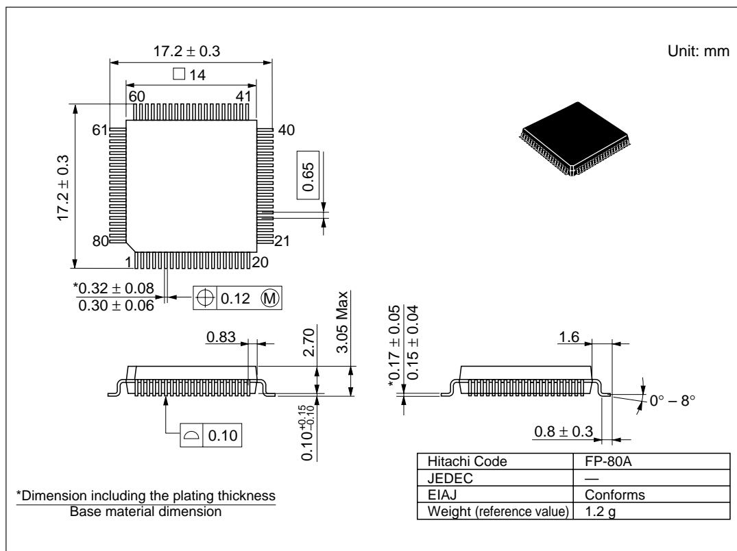
Figure F-1 FP-80A Package Dimensions
