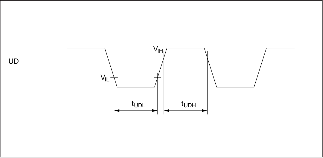
Figure 15-4 UD Pin Minimum Modulation Width Timing
