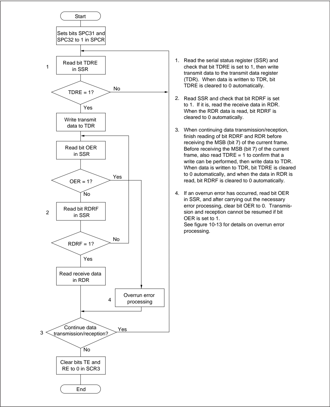
Figure 10-15 Example of Simultaneous Data Transmission/Reception Flowchart(Synchronous Mode)
