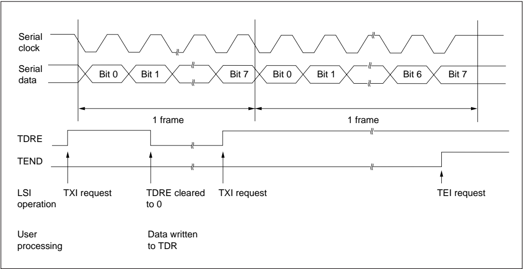
Figure 10-12 Example of Operation when Transmitting in Synchronous Mode
