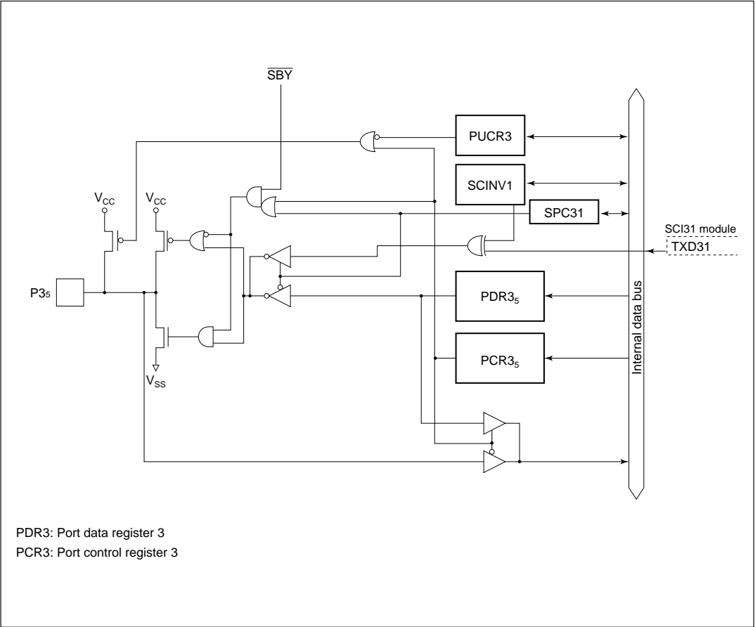
Figure C.2 (b) Port 3 Block Diagram (Pin P3 5 )
