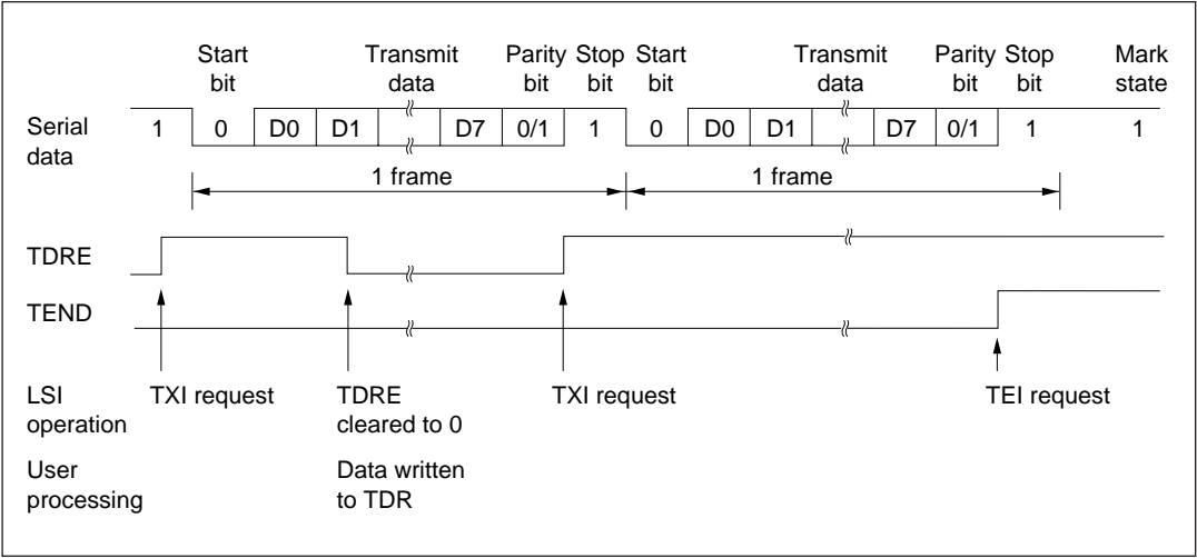
Figure 10-7 Example of Operation when Transmitting in Asynchronous Mode (8-bit data, parity, 1 stop bit)
