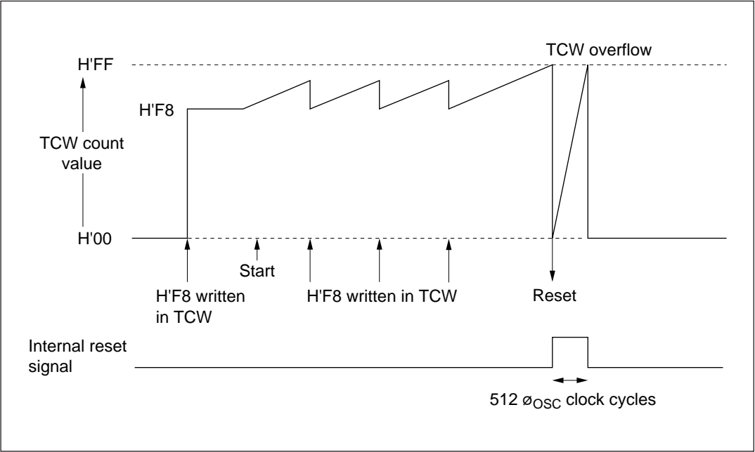
Figure 9-17 Typical Watchdog Timer Operations (Example)
