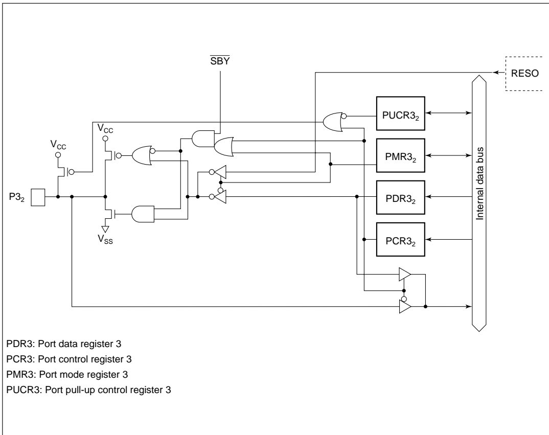
Figure C.2 (e) Port 3 Block Diagram (Pin P3 2 )
