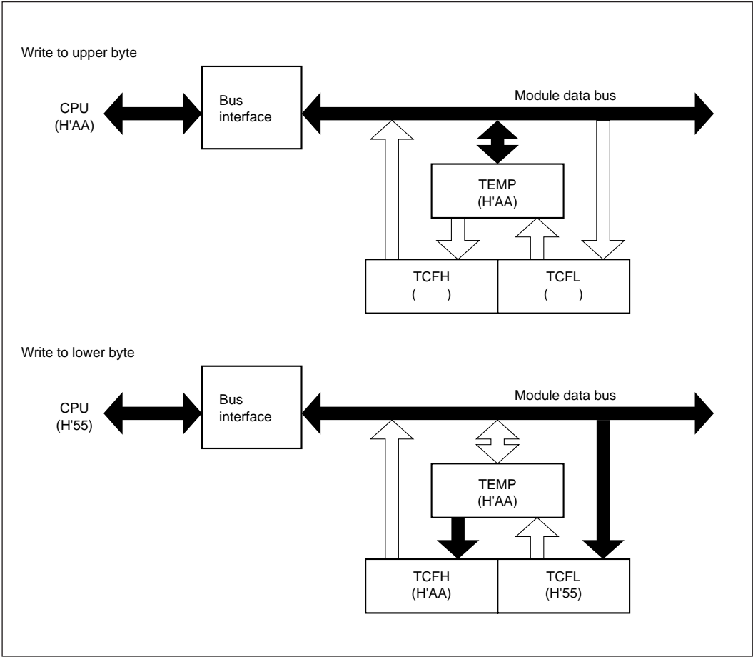
Figure 9-4 Write Access to TCR (CPU → TCF)
