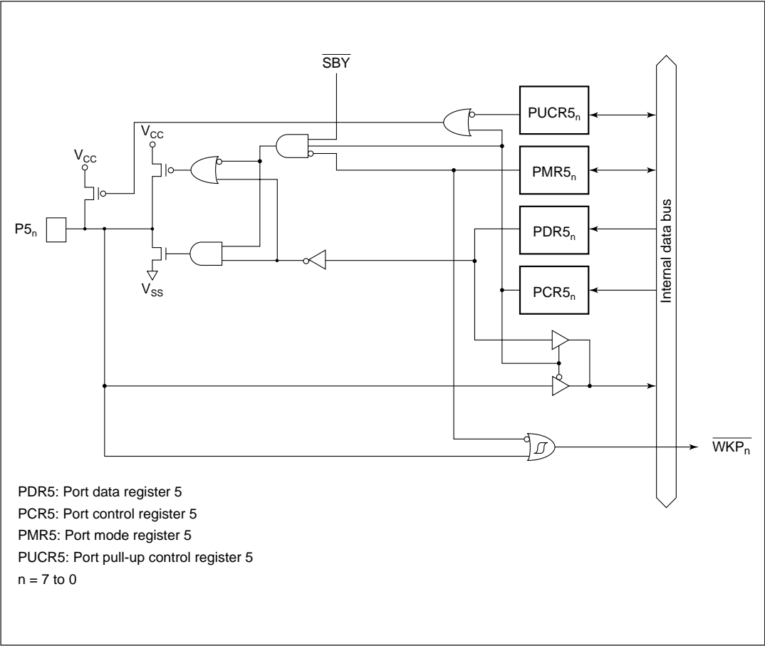
Figure C.4 Port 5 Block Diagram
