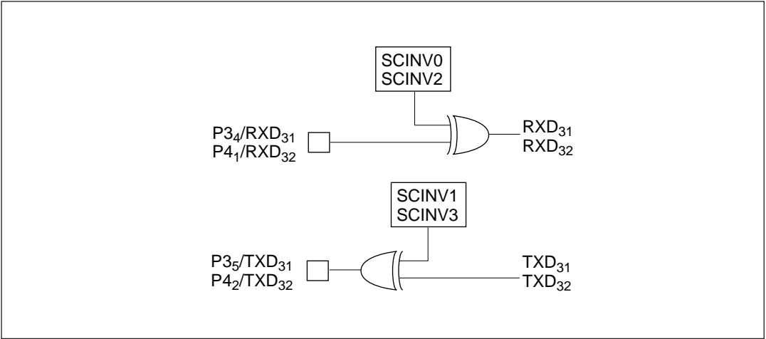
Figure 8.10 Input/Output Data Inversion Function
