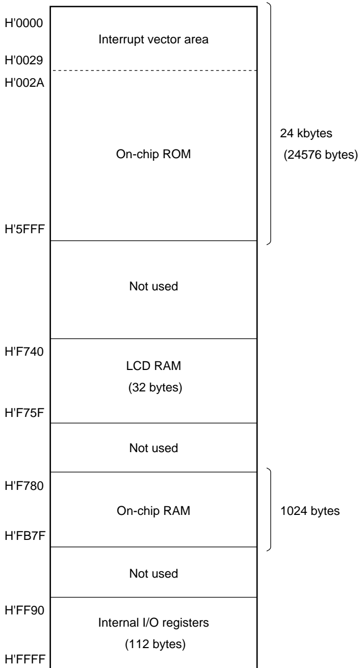
Figure 2-16 (2) H8/3863 and H8/3823 Memory Map
