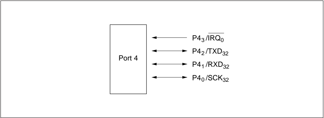
Figure 8-3 Port 4 Pin Configuration
