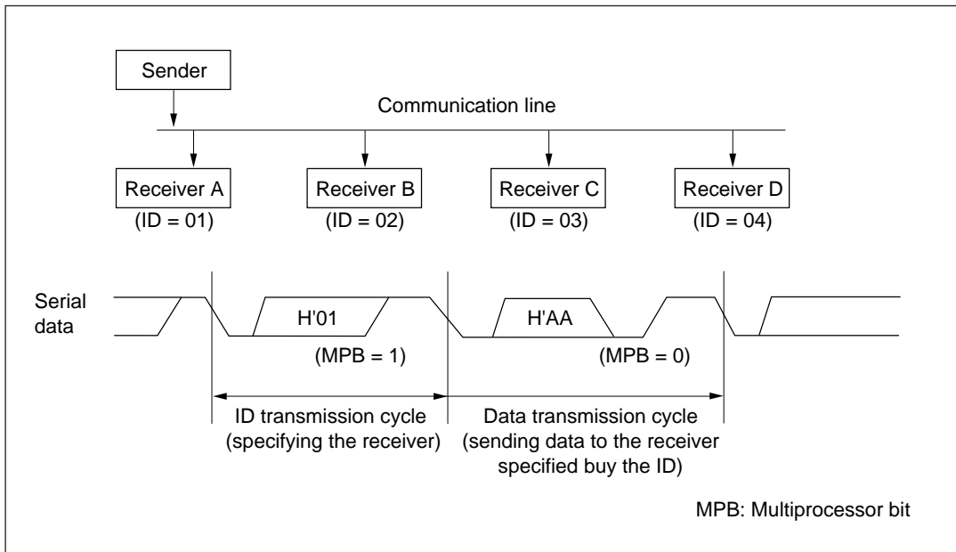
Figure 10-16 Example of Inter-Processor Communication Using Multiprocessor Format (Sending data H'AA to receiver A)
