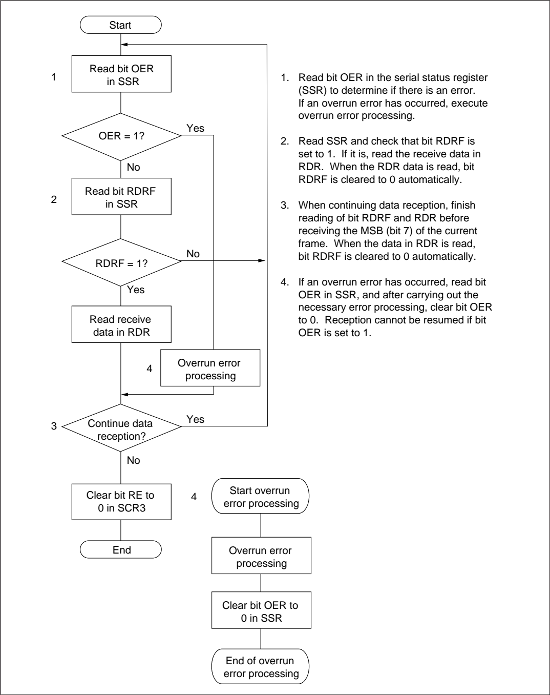
Figure 10-13 Example of Data Reception Flowchart (Synchronous Mode)
