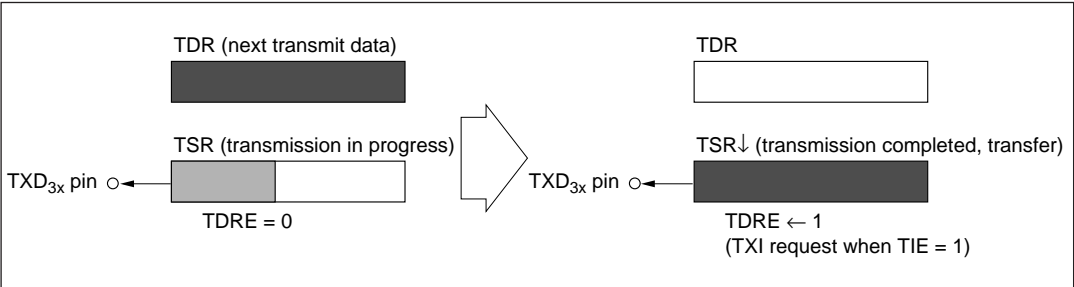
Figure 10-2 (b) TDRE Setting and TXI Interrupt
