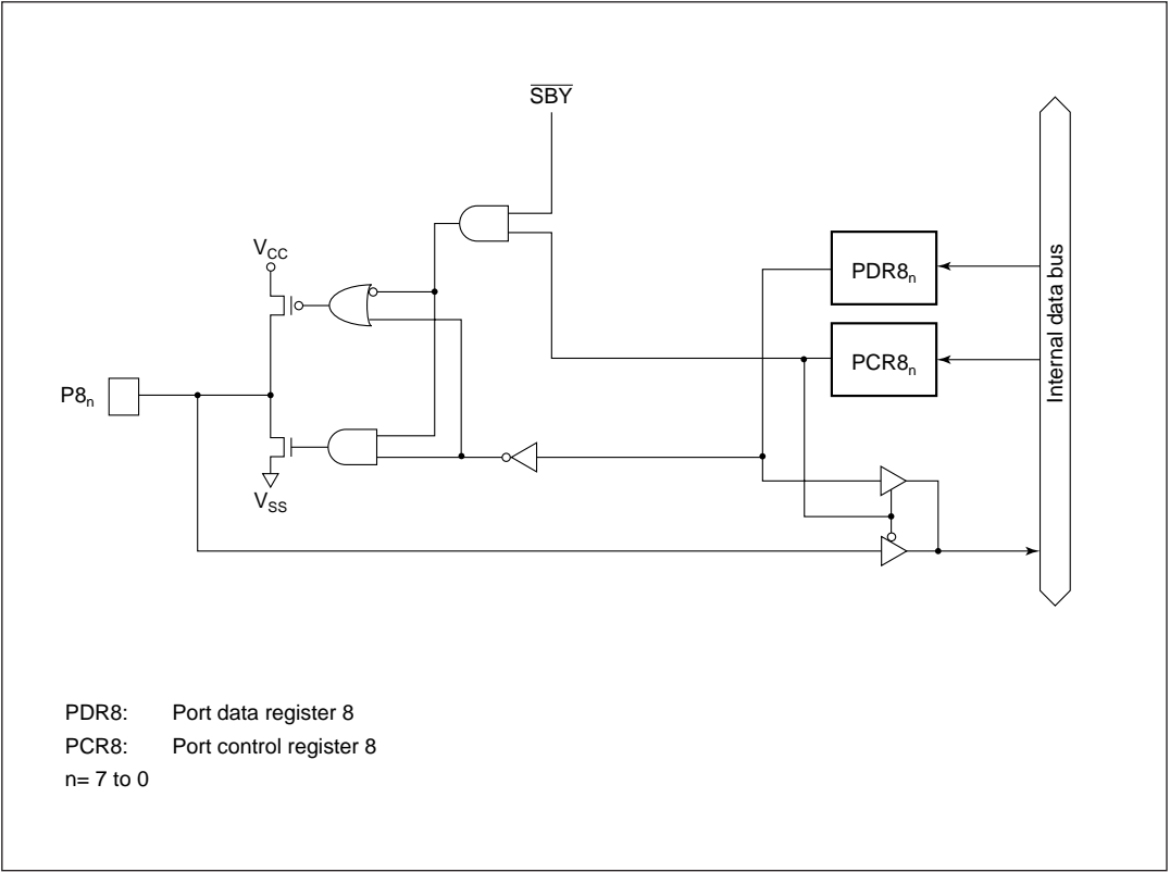
Figure C-7 Port 8 Block Diagram
