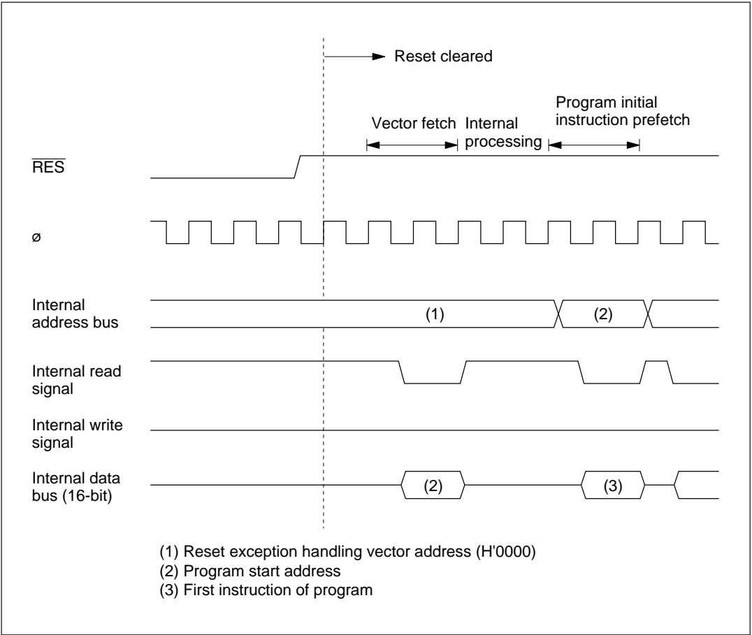
Figure 3-1 Reset Sequence
