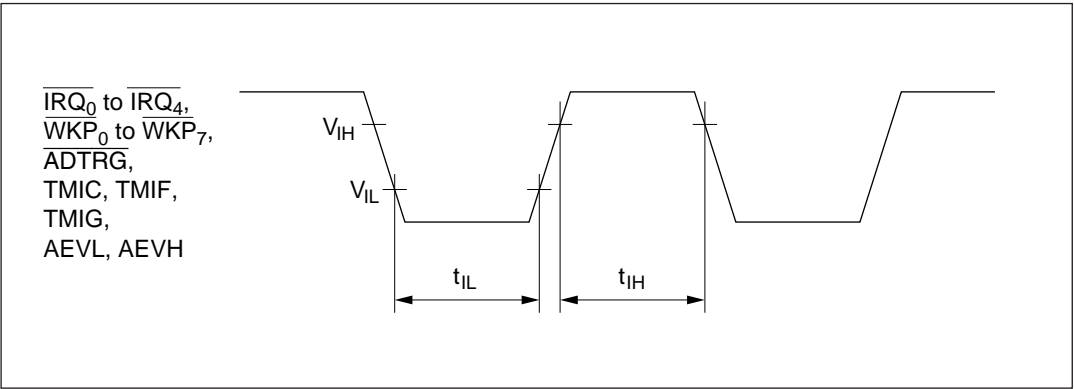
Figure 15-3 Input Timing
