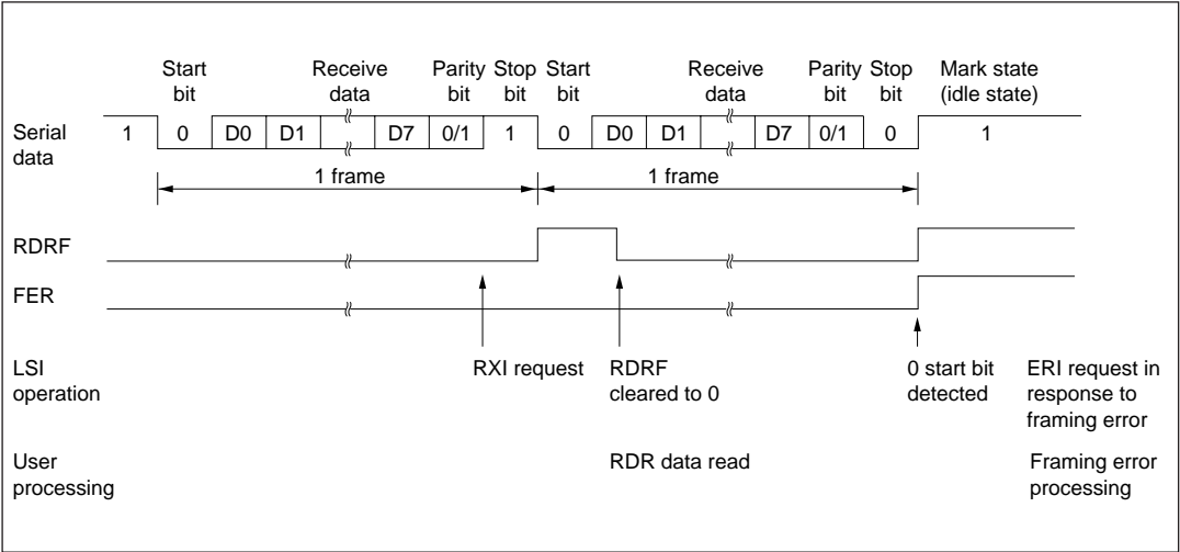
Figure 10-9 Example of Operation when Receiving in Asynchronous Mode (8-bit data, parity, 1 stop bit)
