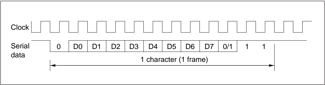
Figure 10-4 Phase Relationship between Output Clock and Transfer Data (Asynchronous Mode) (8-bit data, parity, 2 stop bits)
