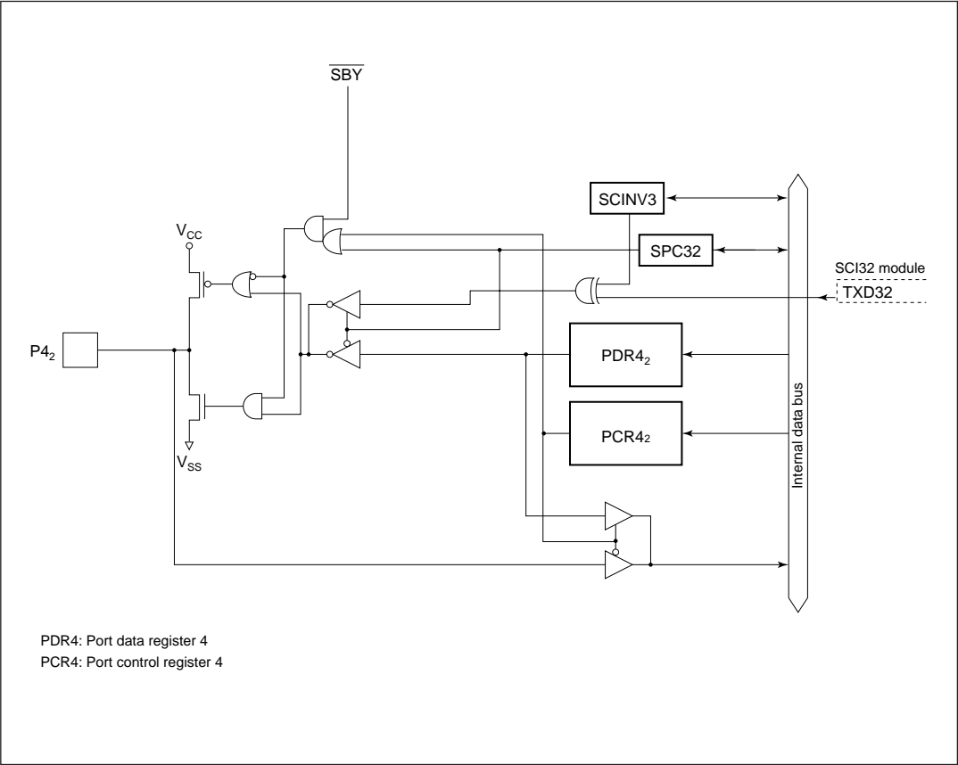
Figure C.3 (b) Port 4 Block Diagram (Pin P4 2 )
