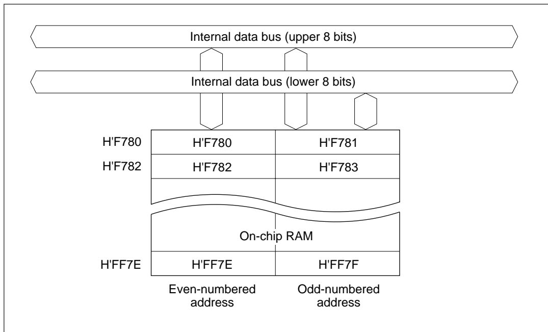
Figure 7-1 RAM Block Diagram (H8/3864 and H8/3824)
