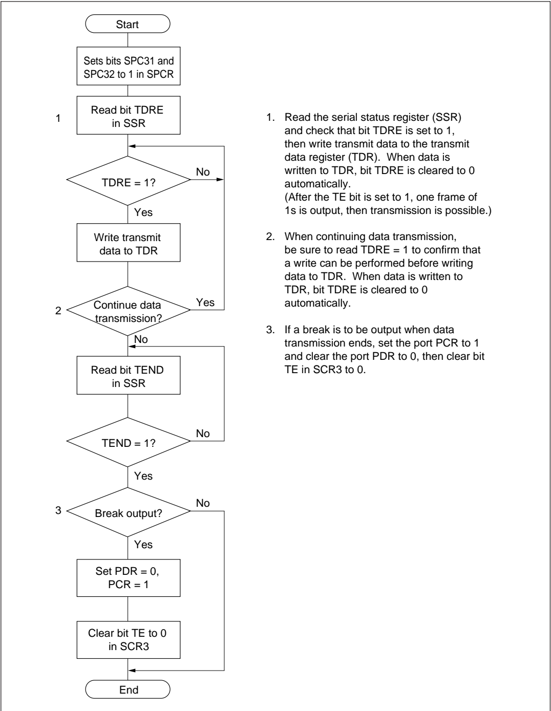
Figure 10-6 Example of Data Transmission Flowchart (Asynchronous Mode)
