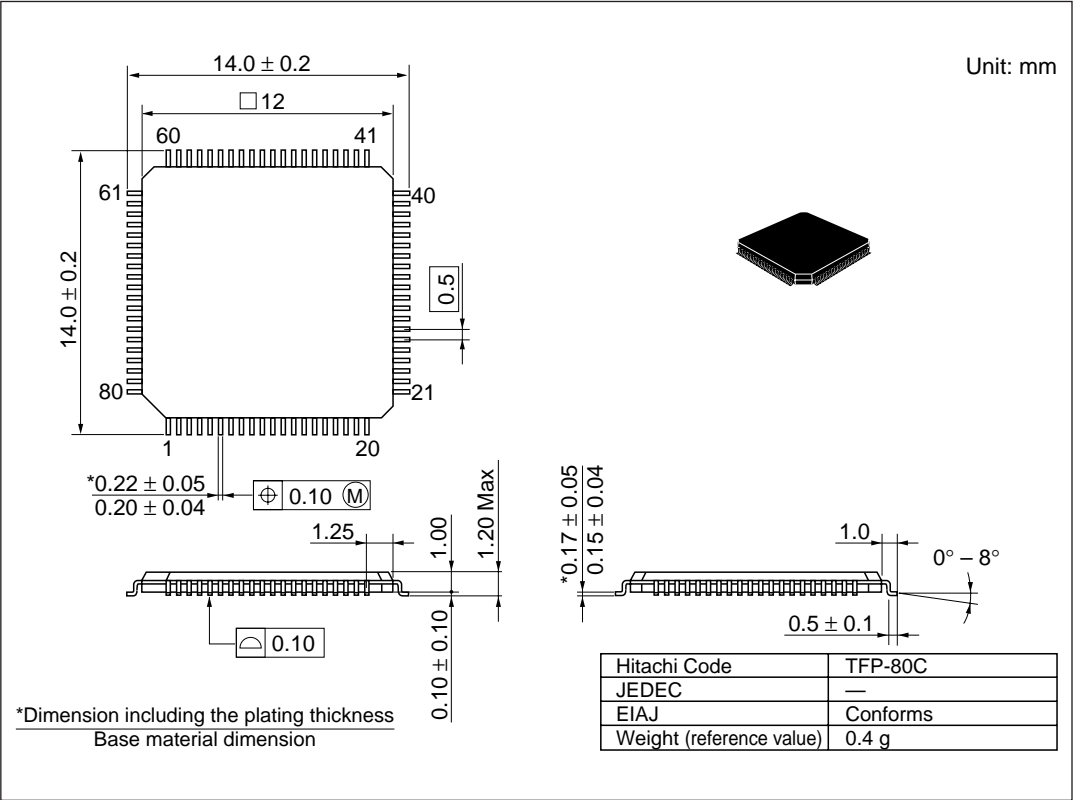
Figure F-3 TFP-80C Package Dimensions
