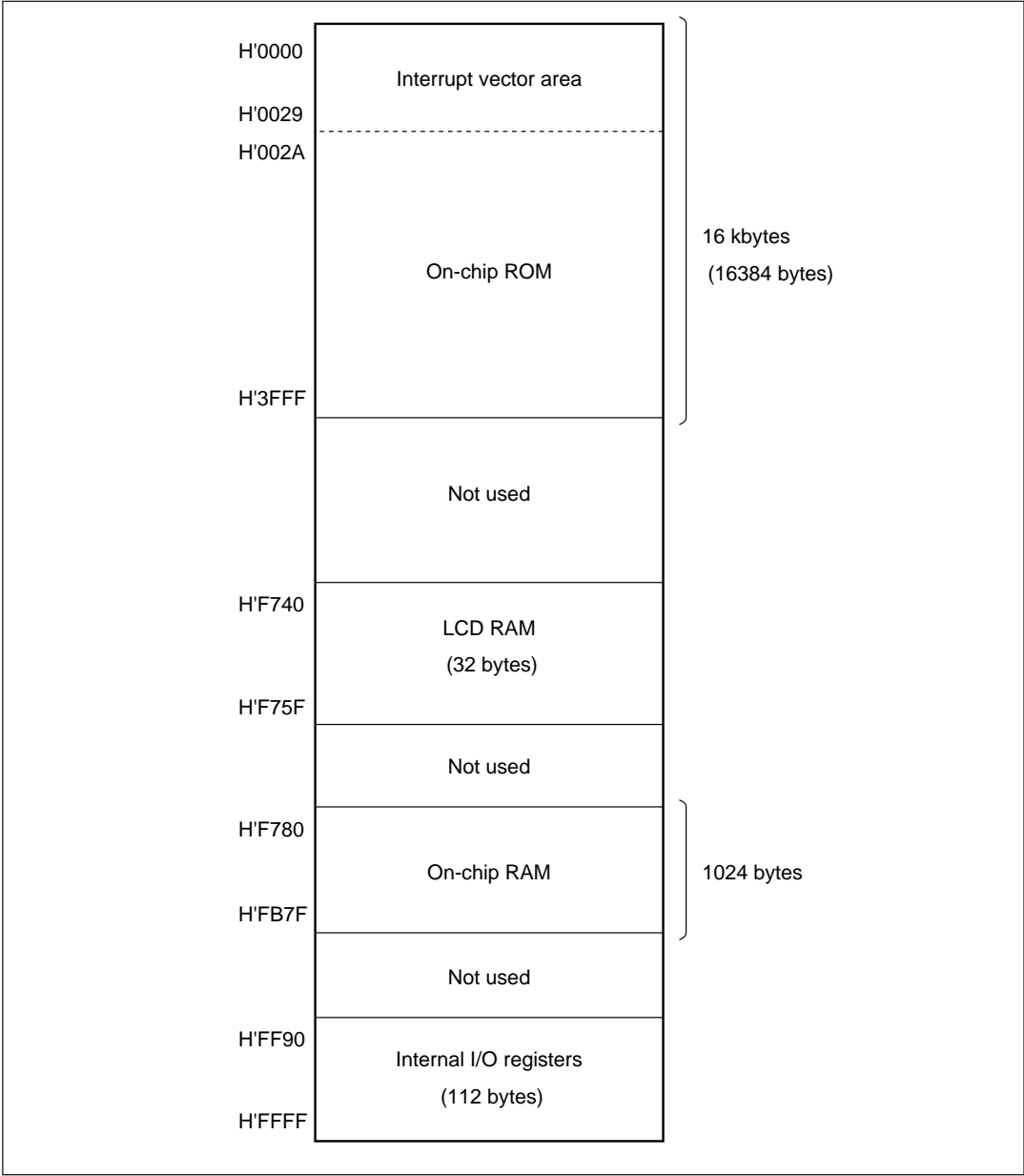
Figure 2-16 (1) H8/3862 and H8/3822 Memory Map
