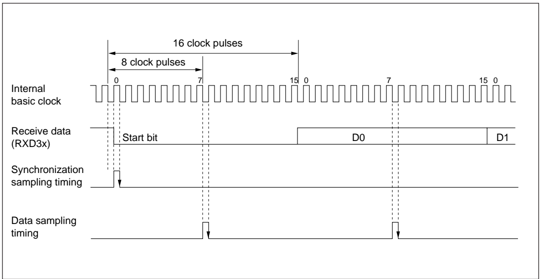
Figure 10-21 Receive Data Sampling Timing in Asynchronous Mode
