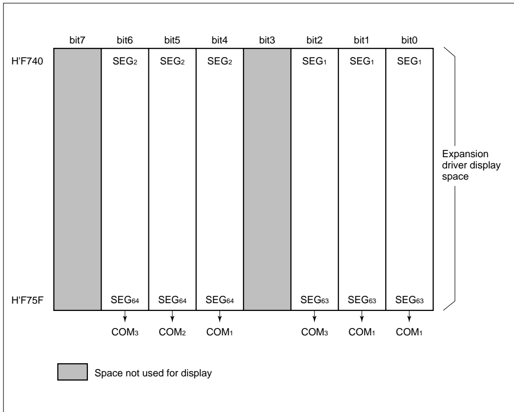
Figure 13-10 LCD RAM Map when Using Segment External Expansion (SGX = "1", SGS3 to SGS0 = "0000" 1/3 Duty)
