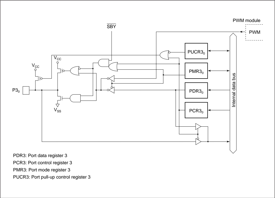
Figure C-2 (g) Port 3 Block Diagram (Pin P3 0 )
