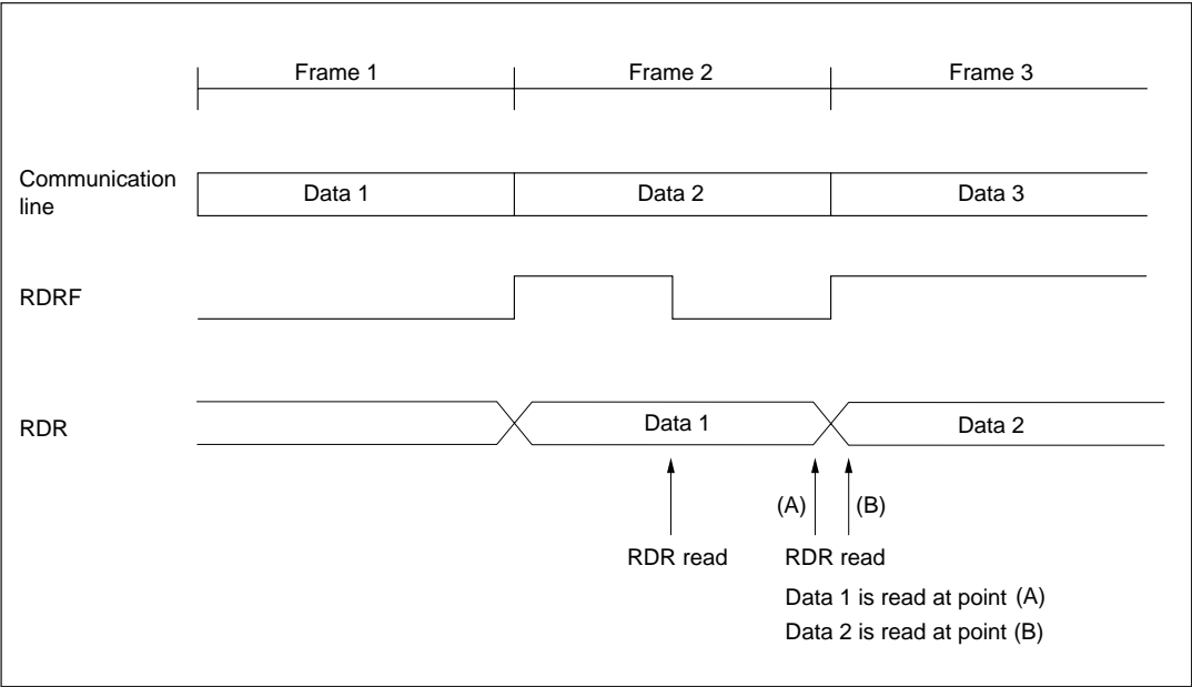
Figure 10-22 Relation between RDR Read Timing and Data
