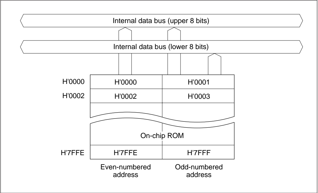
Figure 6-1 ROM Block Diagram (H8/3864 and H8/3824)
