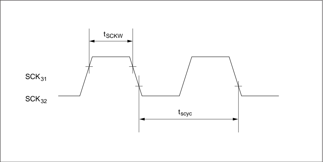
Figure 15-5 SCK3 Input Clock Timing
