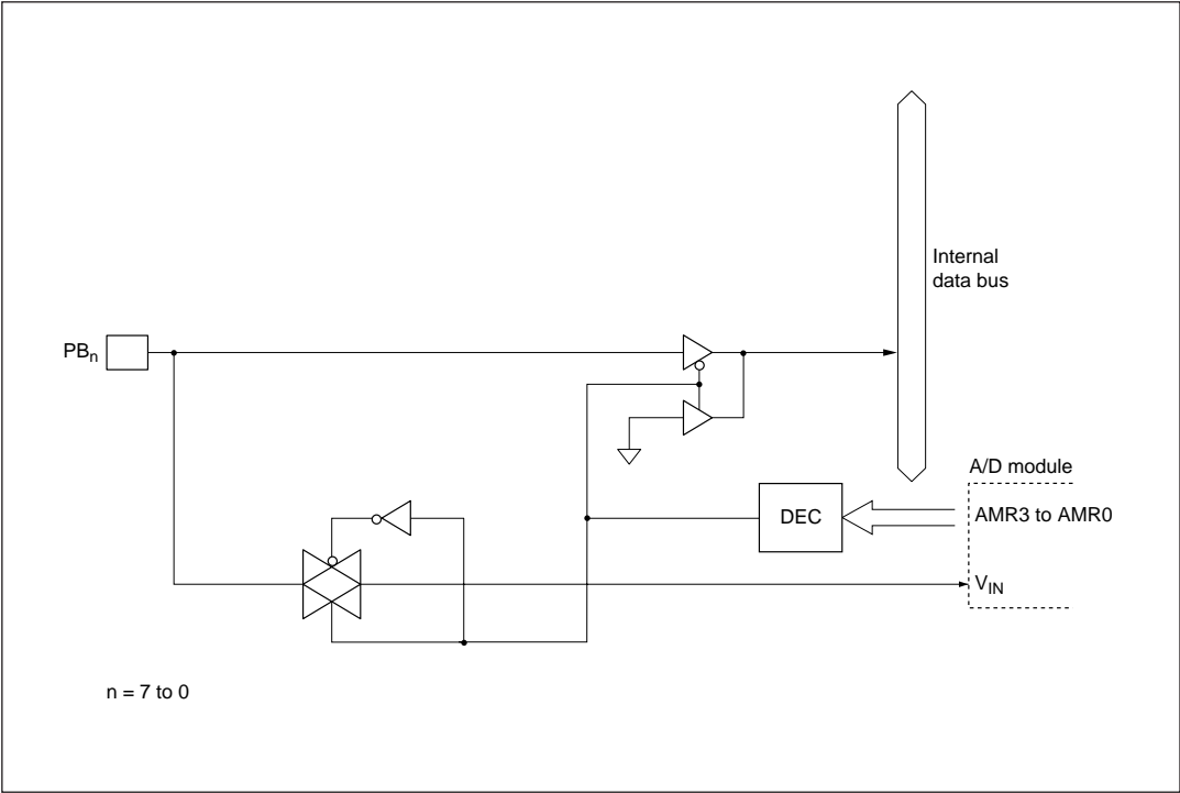
Figure C-9 Port B Block Diagram
