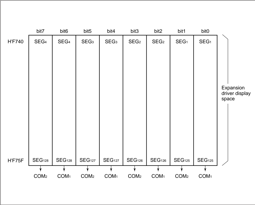
Figure 13-11 LCD RAM Map when Using Segment External Expansion (SGX = “1”, SGS3 to SGS0 = “0000” 1/2 Duty)
