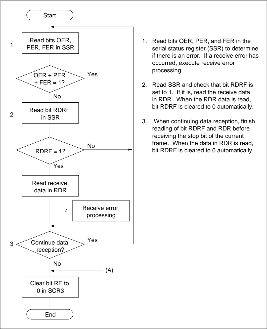
Figure 10-8 Example of Data Reception Flowchart (Asynchronous Mode)
