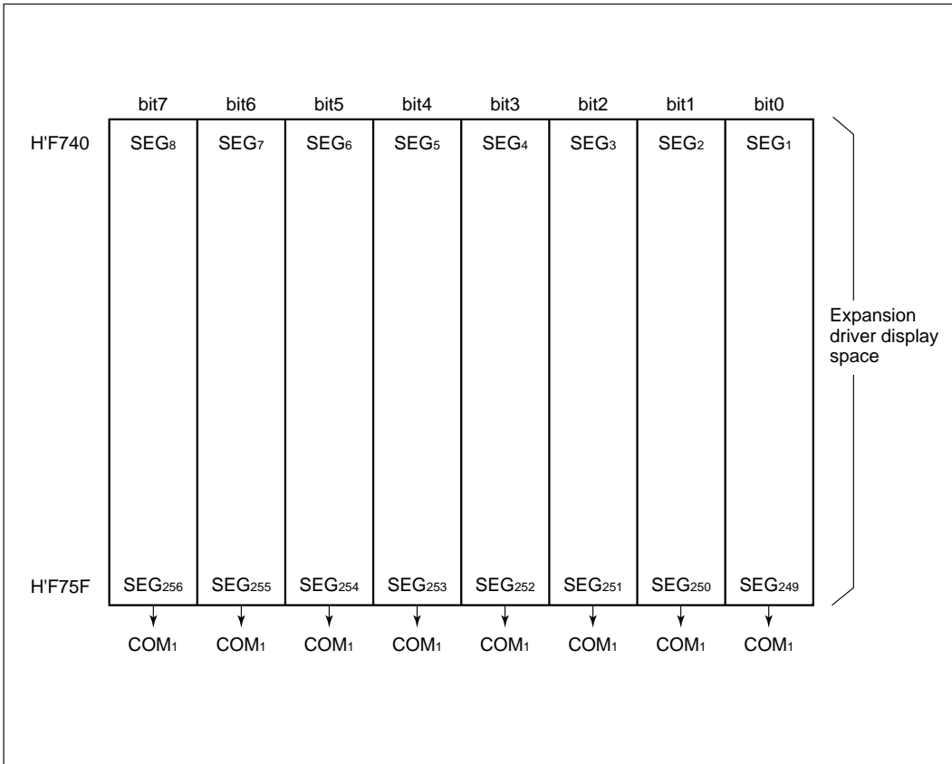
Figure 13-12 LCD RAM Map when Using Segment External Expansion (SGX = "1", SGS3 to SGS0 = "0000" Static)
