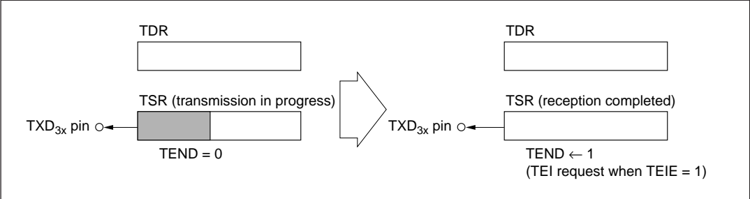
Figure 10-2 (c) TEND Setting and TEI Interrupt
