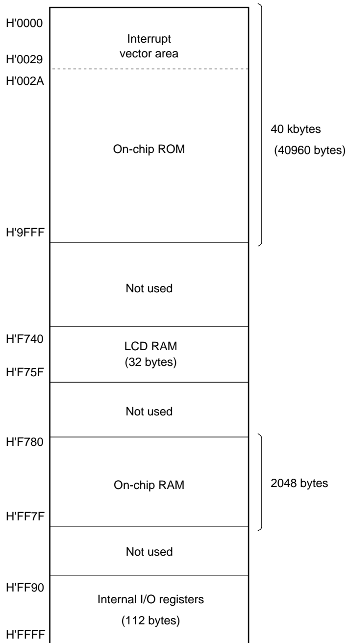
Figure 2-16 (4) H8/3865 and H8/3825 Memory Map
