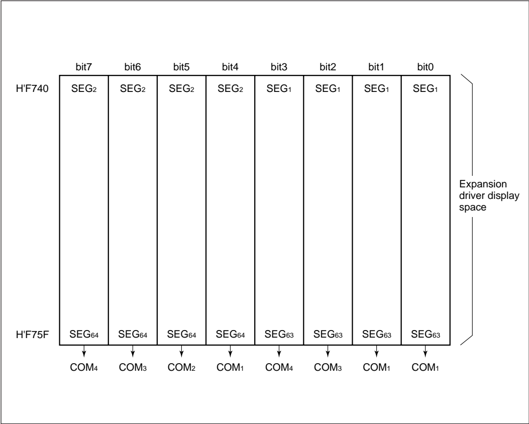
Figure 13-9 LCD RAM Map when Using Segment External Expansion (SGX = “1”, SGS3 to SGS0 = “0000” 1/4 Duty)
