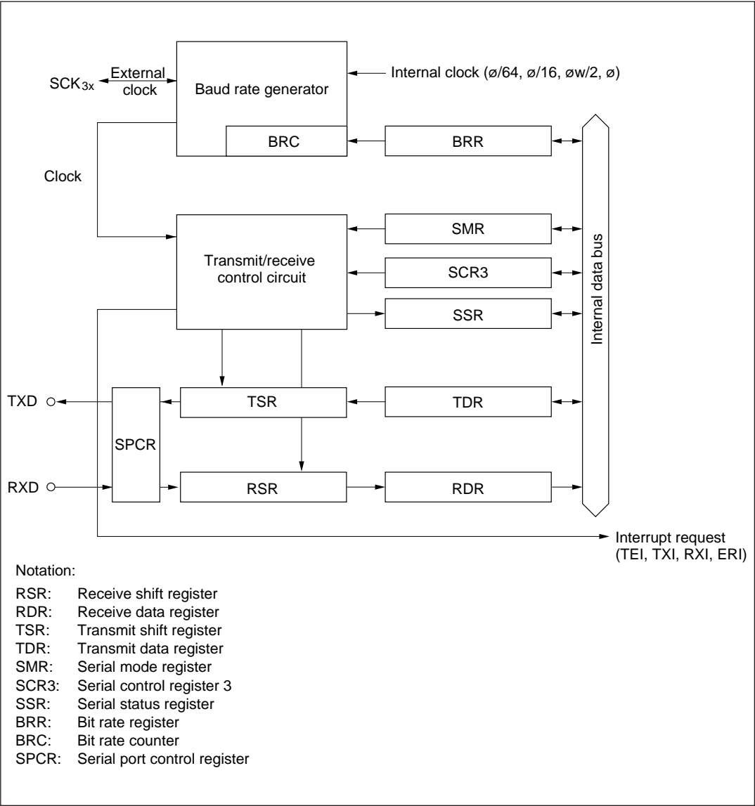
Figure 10-1 SCI3 Block Diagram
