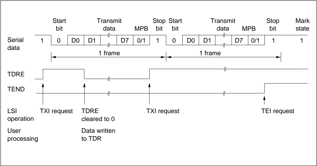
Figure 10-18 Example of Operation when Transmitting using Multiprocessor Format (8-bit data, multiprocessor bit, 1 stop bit)
