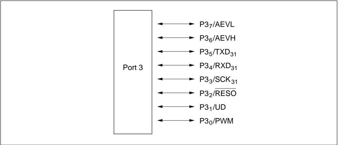
Figure 8-2 Port 3 Pin Configuration
