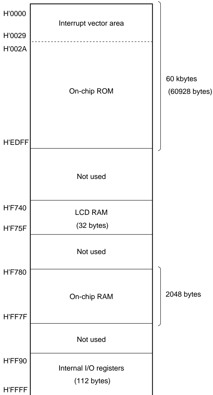
Figure 2-16 (6) H8/3867 and H8/3827 Memory Map
