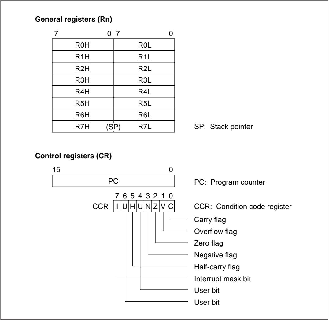
Figure 2-1 CPU Registers
