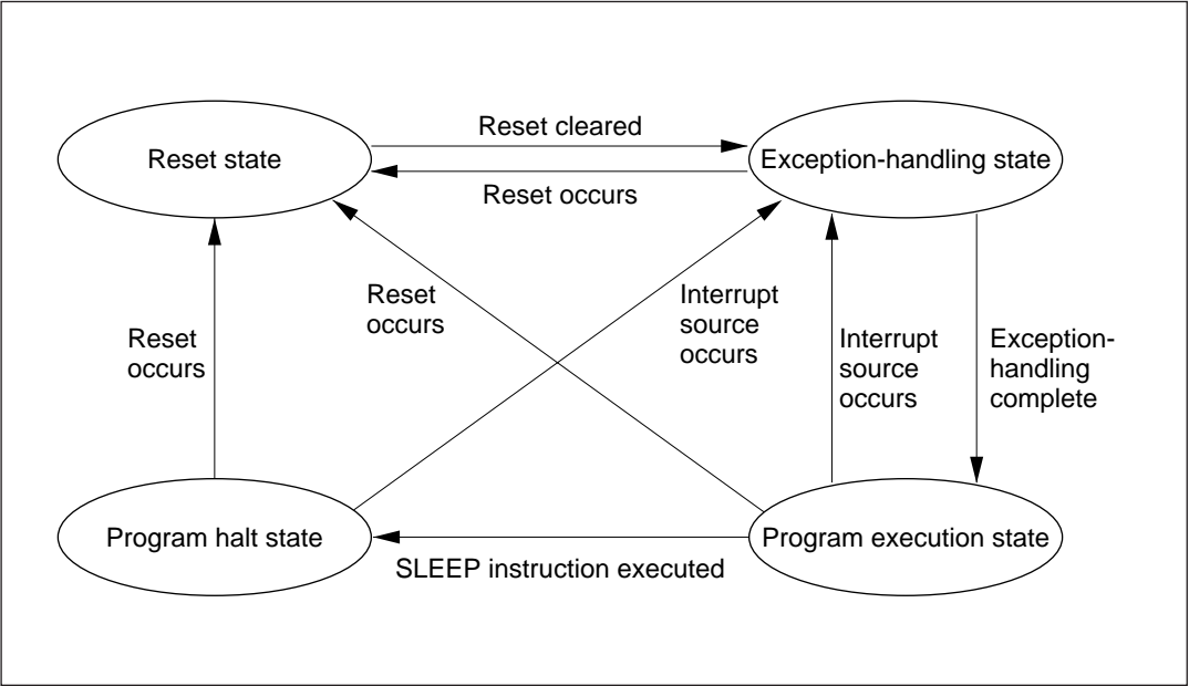
Figure 2-15 State Transitions
