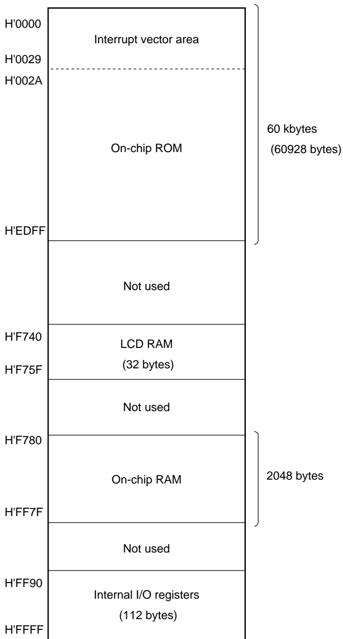
Figure 2-16 (6) H8/3847R Memory Map
