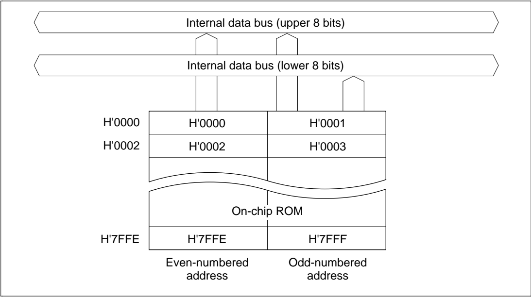
Figure 6-1 ROM Block Diagram (H8/3844R)
