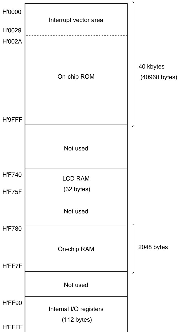
Figure 2-16 (4) H8/3845R Memory Map
