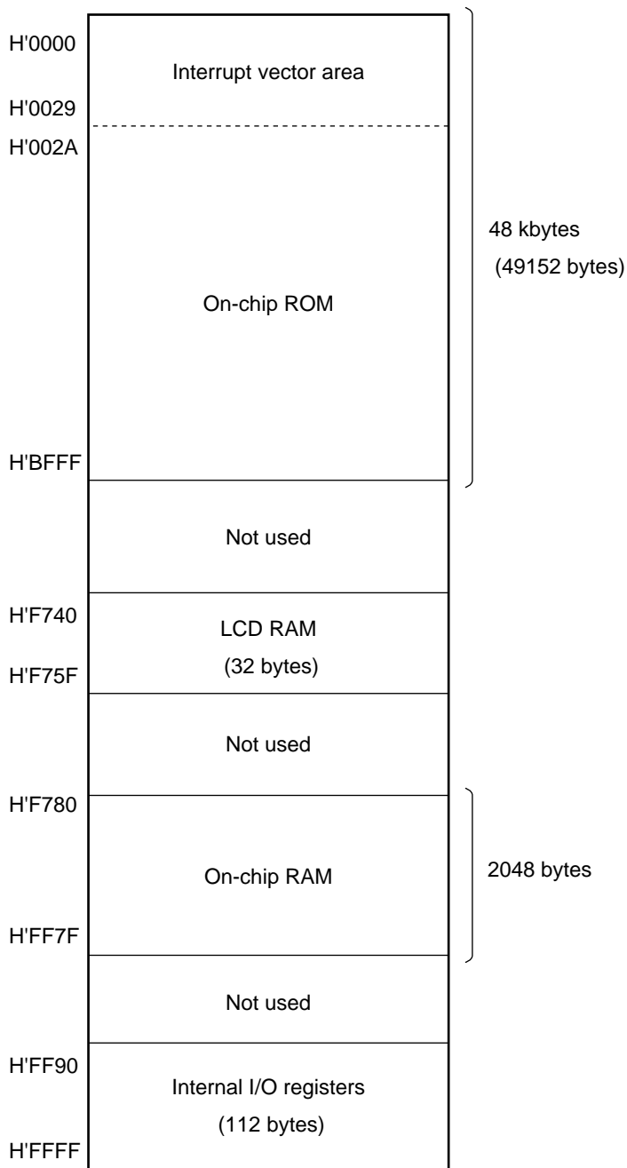
Figure 2-16 (5) H8/3846R Memory Map
