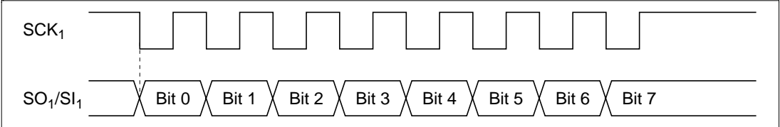
Figure 10-2 Transfer Format
