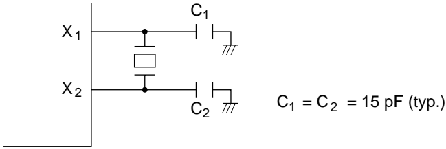
Figure 4-7 Typical Connection to 32.768-kHz/38.4 kHz Crystal Oscillator (Subclock)
