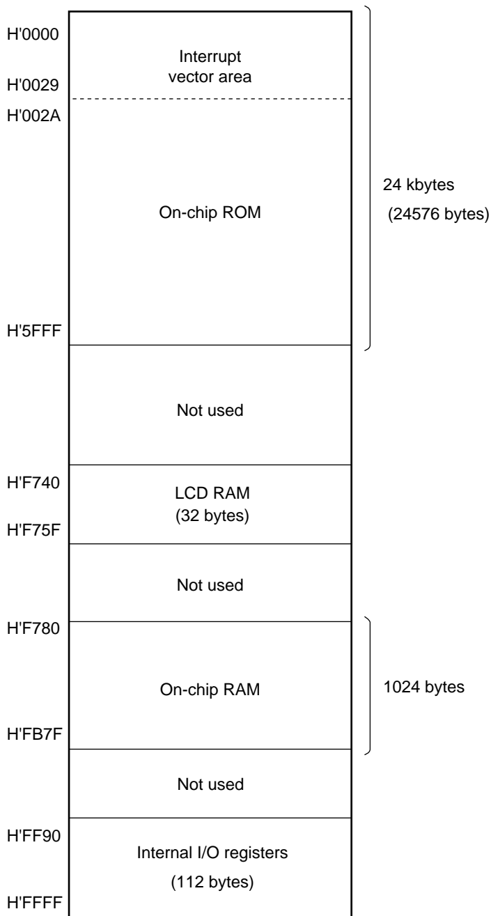
Figure 2-16 (2) H8/3843R Memory Map
