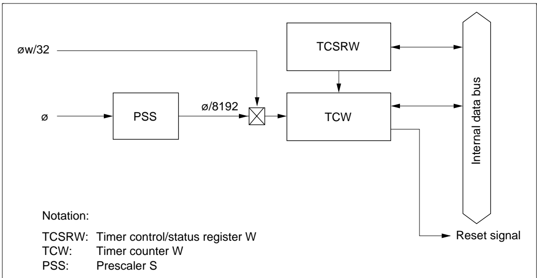
Figure 9-16 Block Diagram of Watchdog Timer
