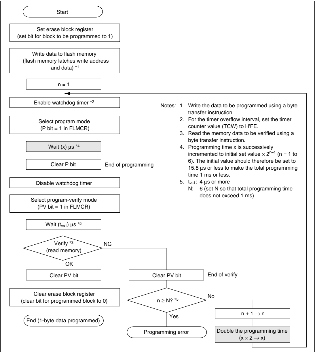
Figure 6.14 Programming Flowchart
