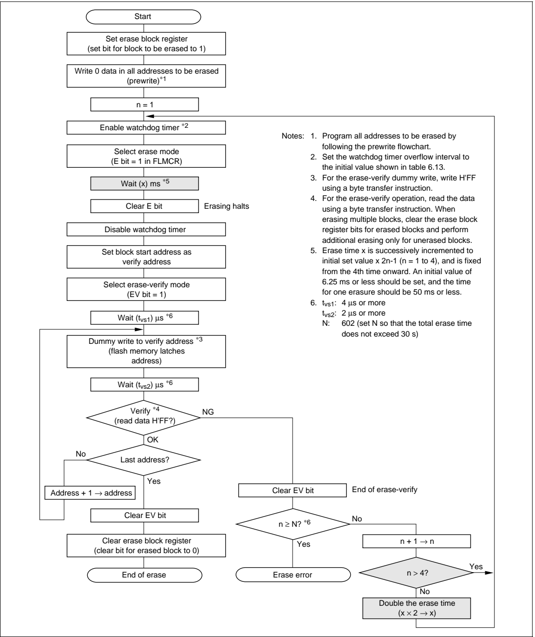
Figure 6.15 Erase Flowchart
