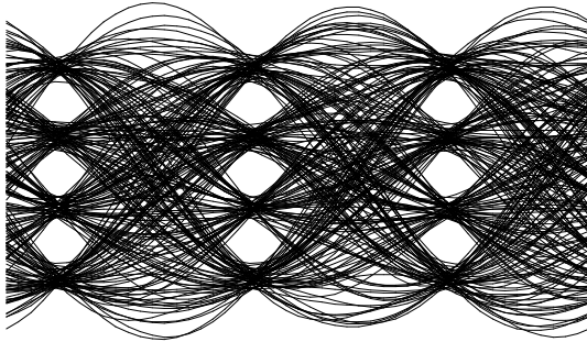
Figure 15b Tx Signal Eye TXIMP = 0
