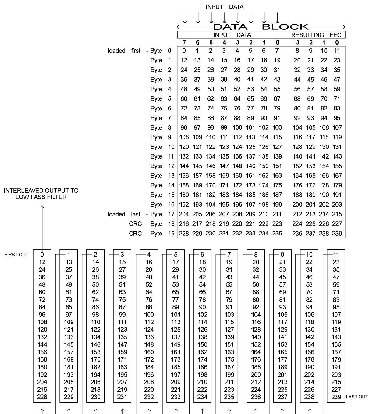
Figure 13 Interleaving - Input/Output
