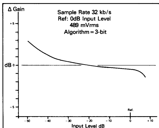
Fig. 6 Typical Variation of Gain with Input Level
