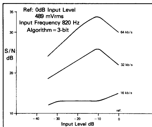
Fig. 7 Typical S/N Ratio with Input Level
