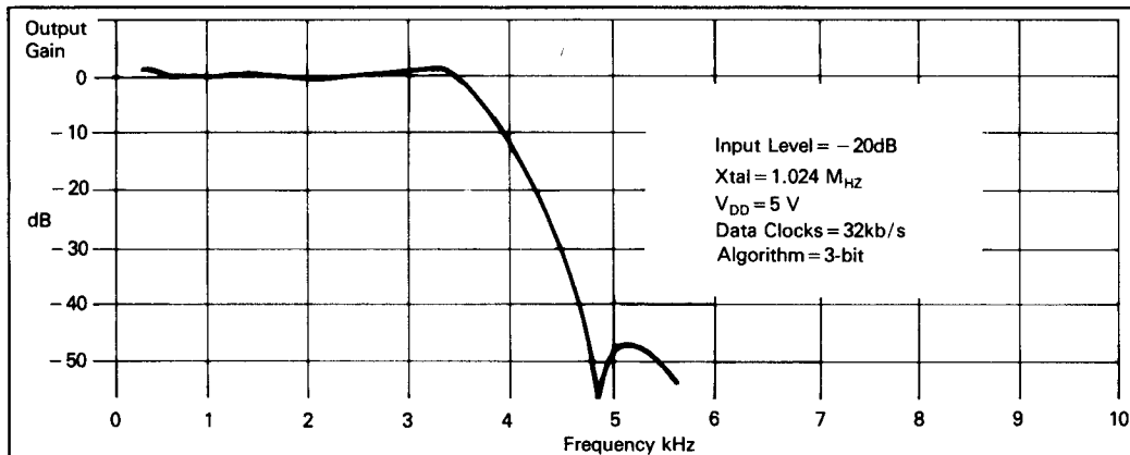
Fig. 5 Typical Codec Frequency Response
