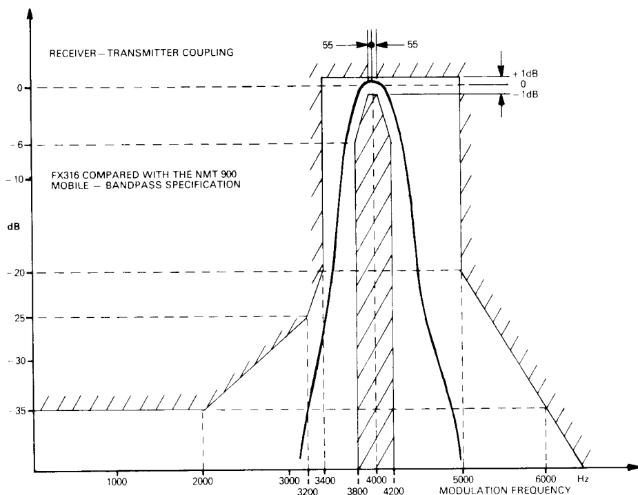
Fig. 5 Typical FX316 4kHz Bandpass Filter Response
