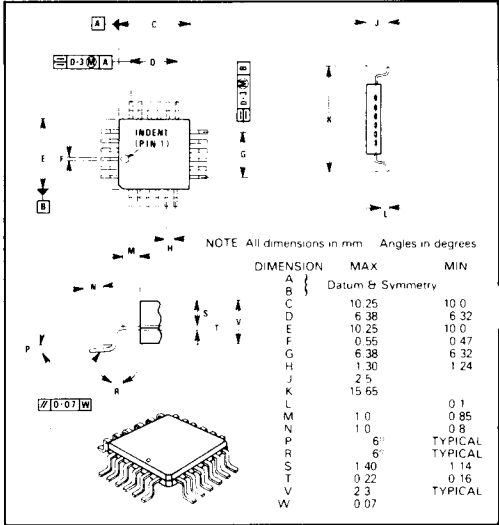
Fig. 8 FX316LH Package
