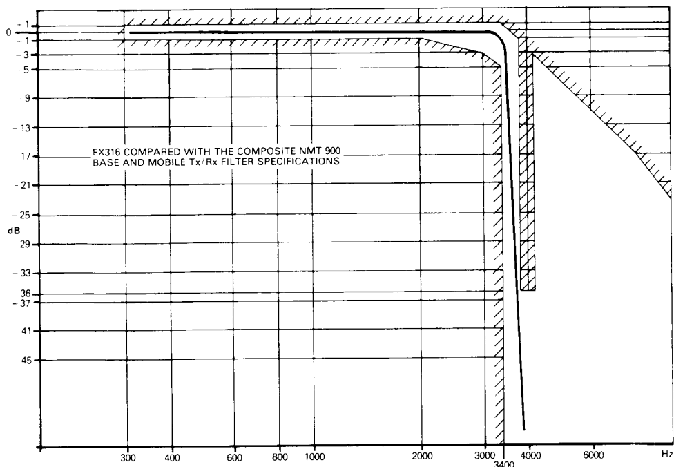
Fig. 4 Typical FX316 Lowpass Filter Response
