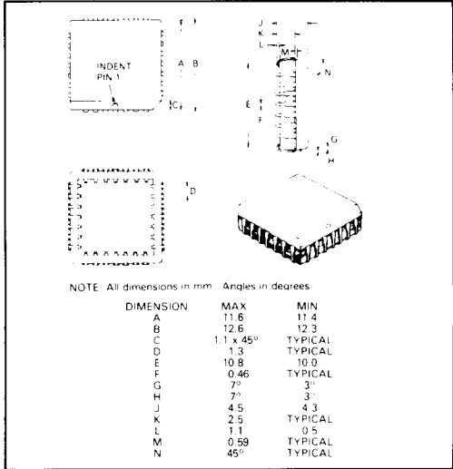
Fig. 8 FX316LH Package
