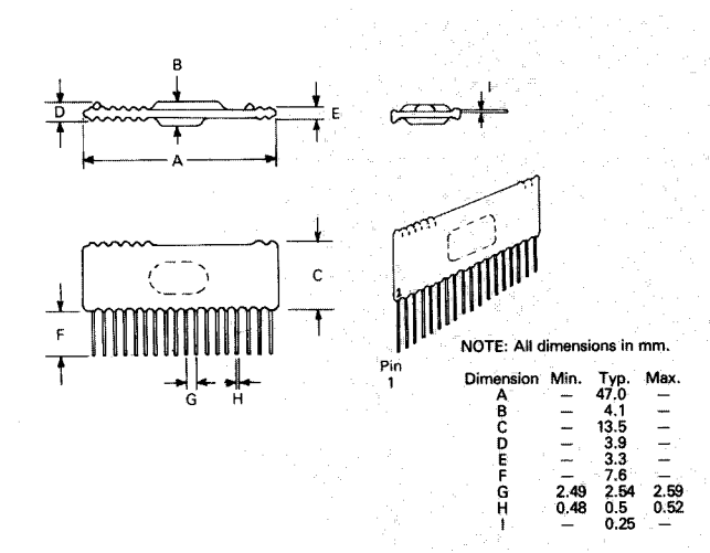
Fig. 3 FX1103 SIL Package
