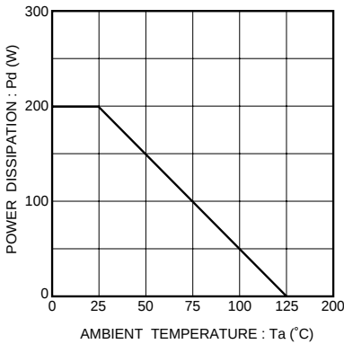
Fig. 1 Derating curve
