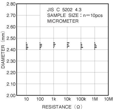
Fig.3 Dimensions (diameter)
