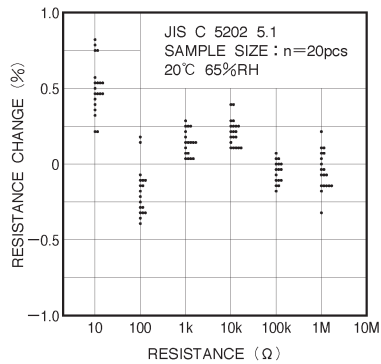
Fig.5 DC resistance
