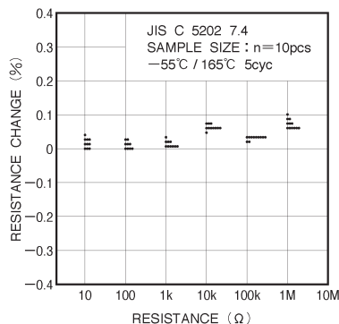
Fig.12 Temperature cycling
