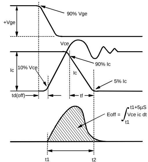
Fig. 18b - Test Waveforms for Circuit of Fig. 18a, Defining E_{off} , t_{d(off)} , t_r
