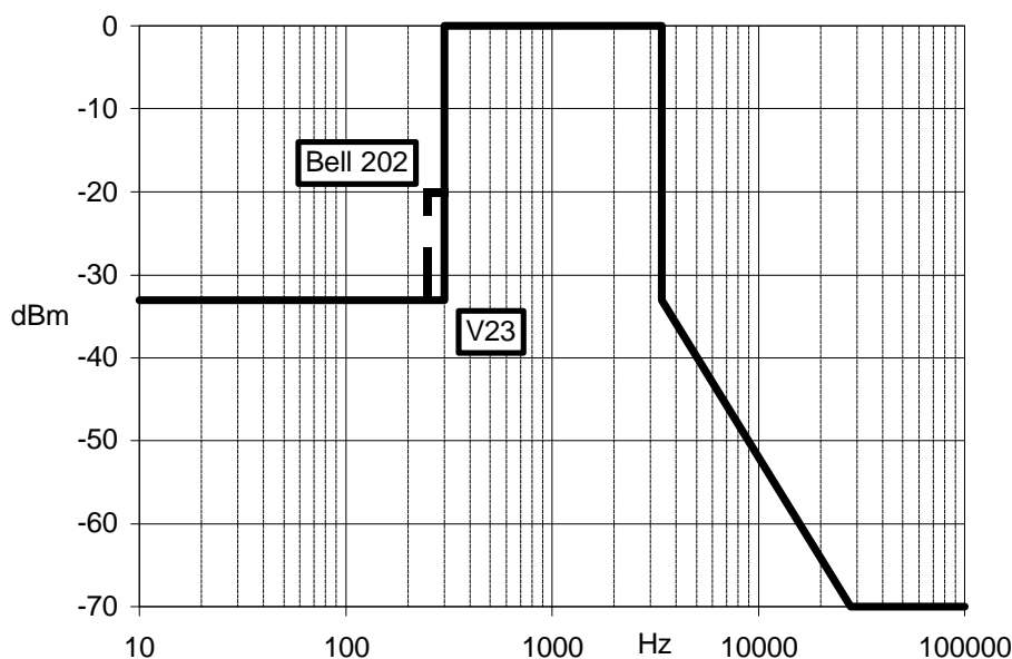
Figure 5 Maximum Out of Band Tx Line Energy Limits
