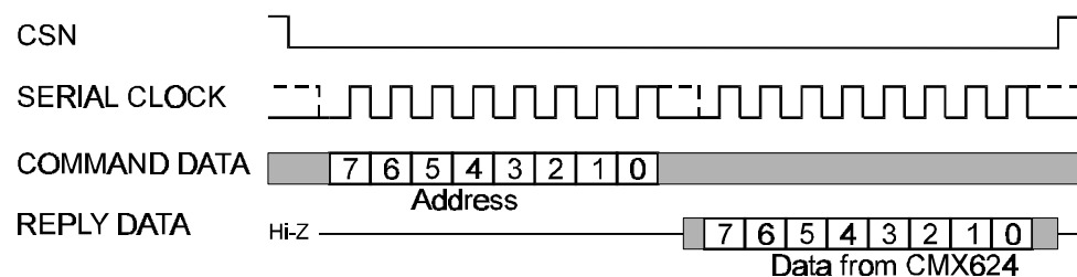
Figure 7 'C-BUS' Transactions
