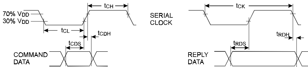
Figure 10 'C-BUS' Timing
