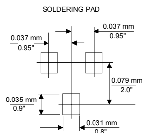
Outline SOT23
