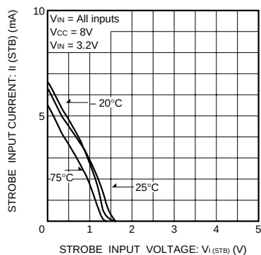
Fig. 21 Strobe terminal input current vs. input voltage
