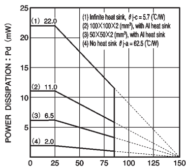
Fig. 6 Ta - power dissipation characteristics (TO220FP)
