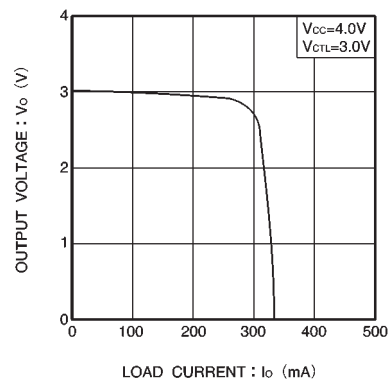
Fig.4 I_o vs. V_o
