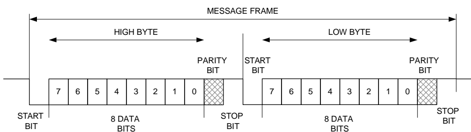
Figure 8. Command Bits
