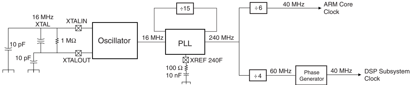
Figure 5. AT75C220 Clocking
