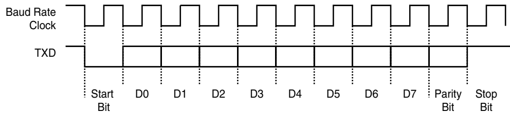
Figure 20. Synchronous and Asynchronous Mode: Character Transmission
