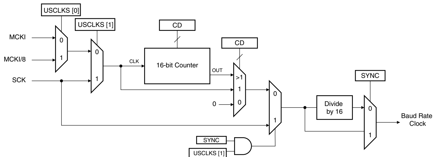
Figure 16. Baud Rate Generator
