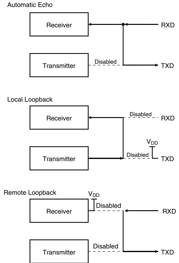
Figure 21. Channel Modes
