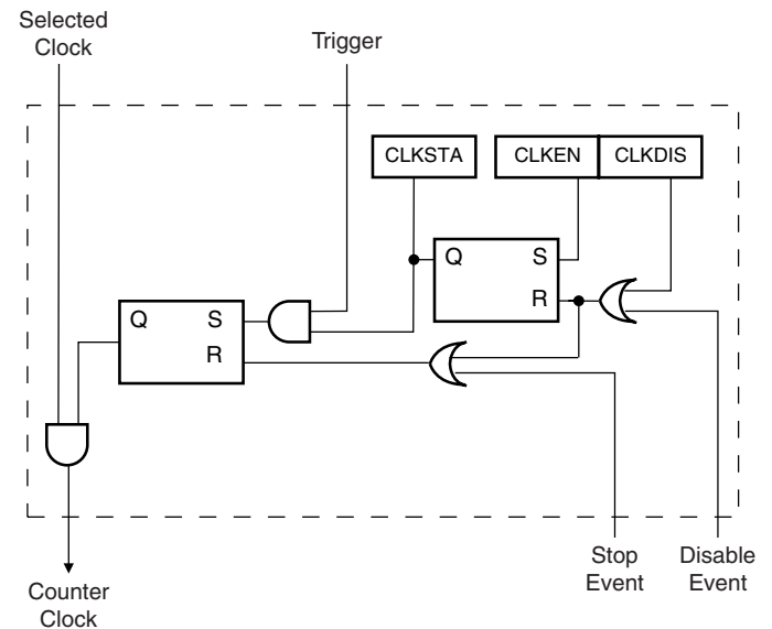
Figure 24. Clock Control
