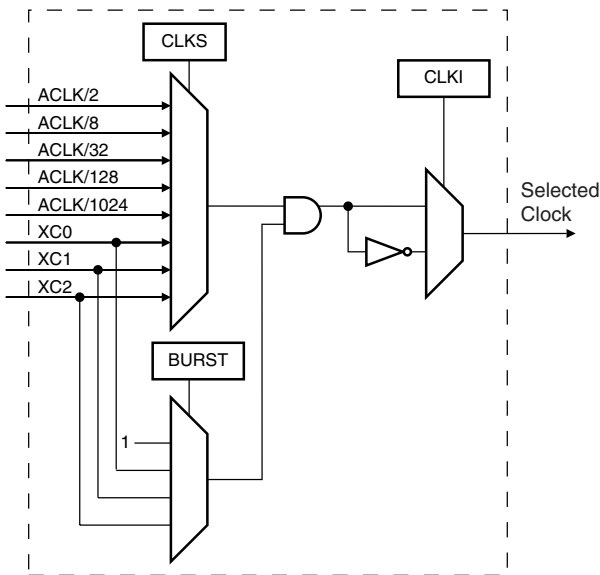
Figure 23. Clock Selection
