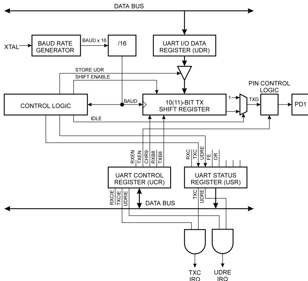
Figure 19. UART Transmitter
