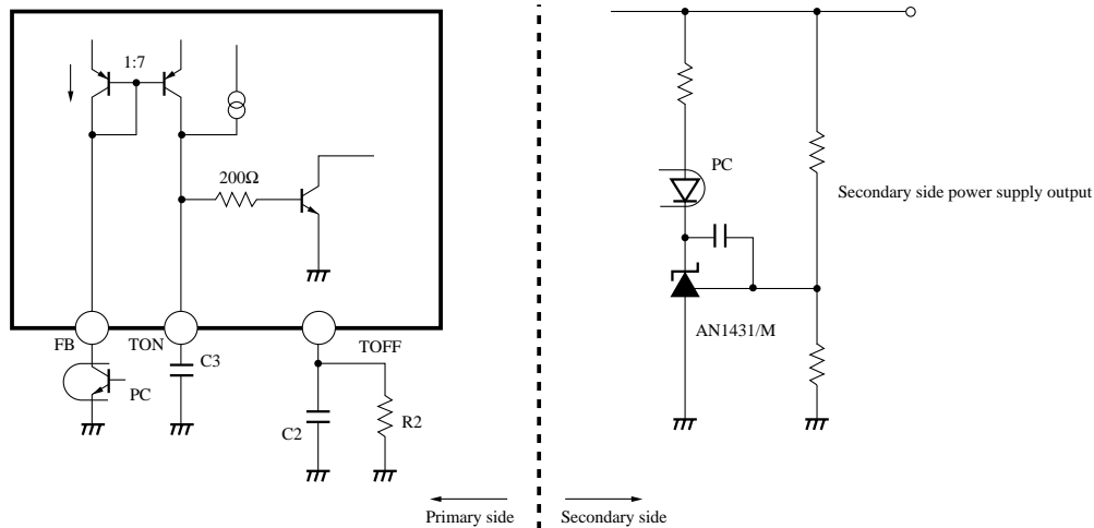
Fig.3 Power Supply Output Control System
