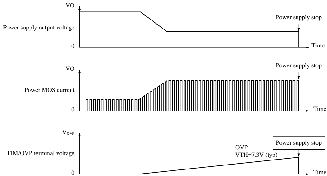
Fig.10 Timer Latch Basic Operation
