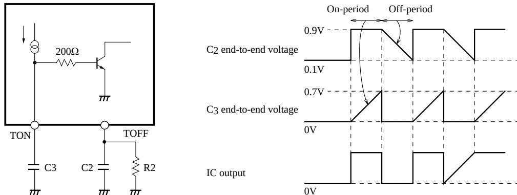
Fig.2 Oscillation Circuit operation
