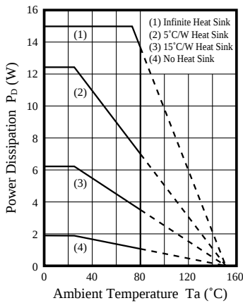
P_D - T_a (AN7900T Series)
