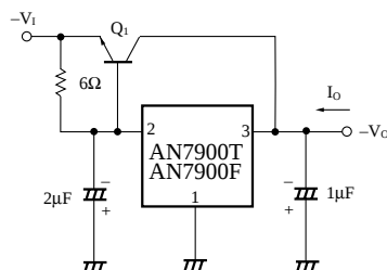
1) Current Boost Circuit
