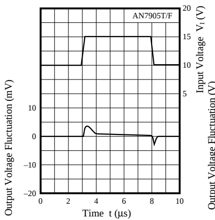
Input Transient Response
