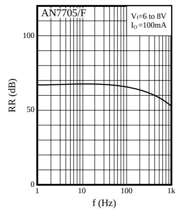
RR - f
