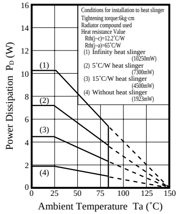
P_D - T_a (AN7700F series)
