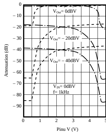
Balance Mode Attenuation Characteristics
