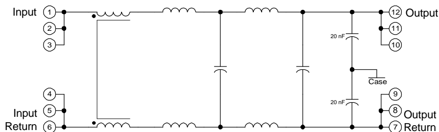
Figure I. AME50461 Block Diagram
