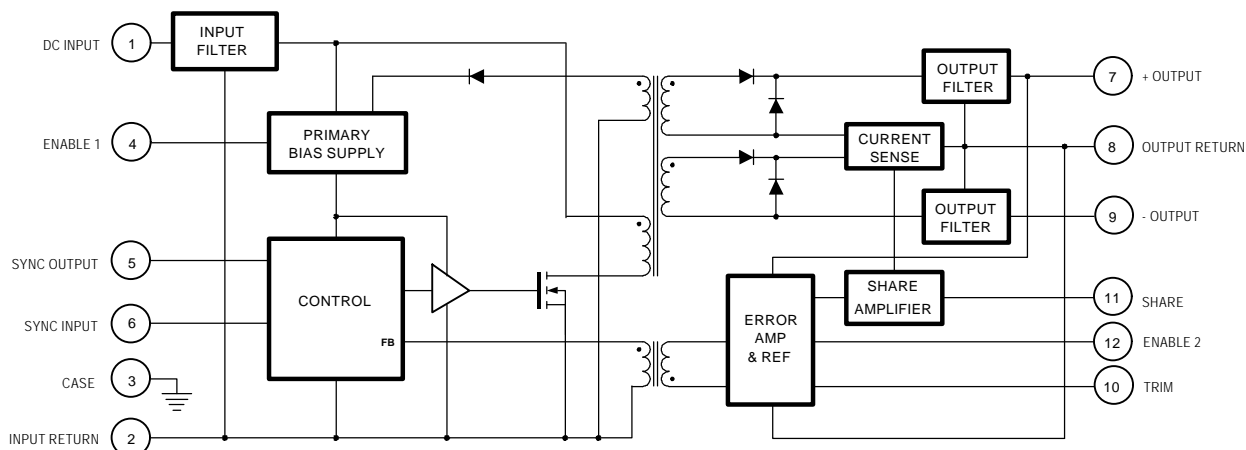
Figure I. AFL Dual Output Block Diagram
