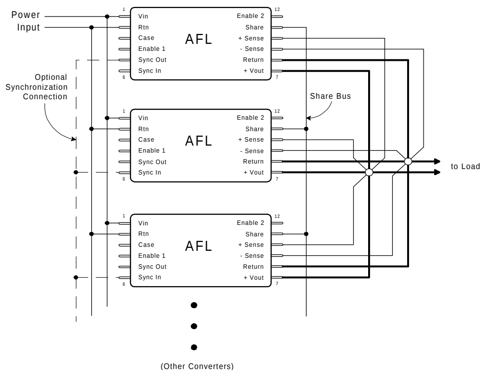
Figure III. Preferred Connection for Parallel Operation
