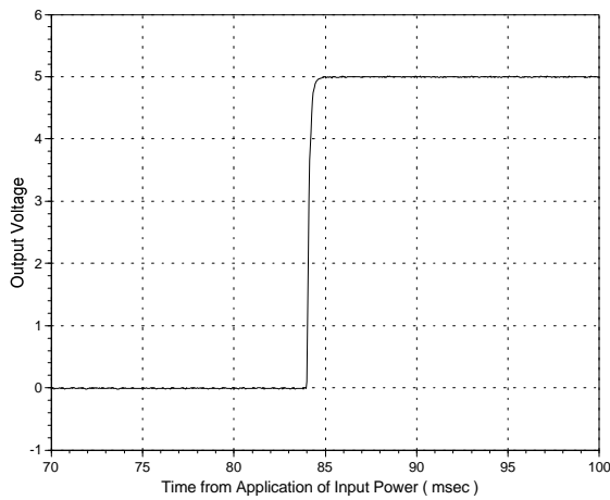
Turn-on Time, No Load
