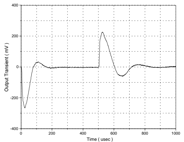
Output Load Transient Response 10% Load to/from 50% Load
