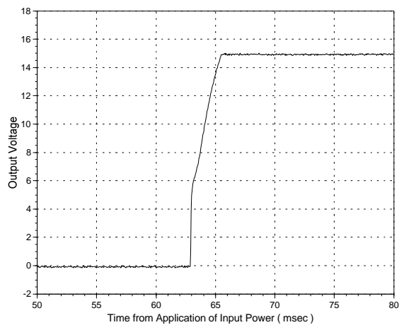
Turn-on Time, Full Load
