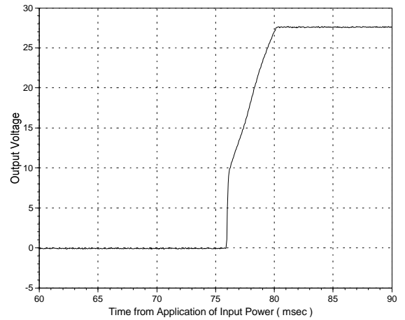
Turn-on Time, Full Load
