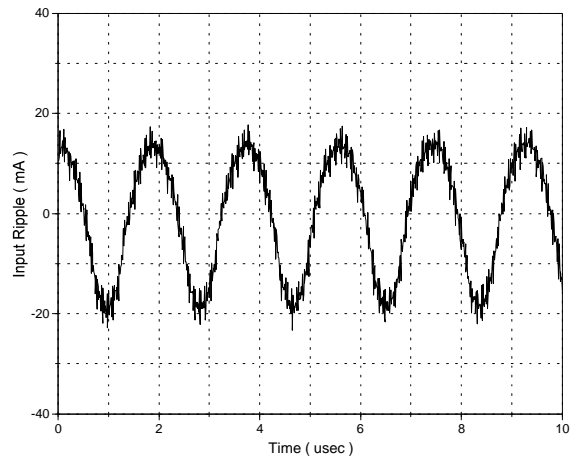
Input Ripple Current
