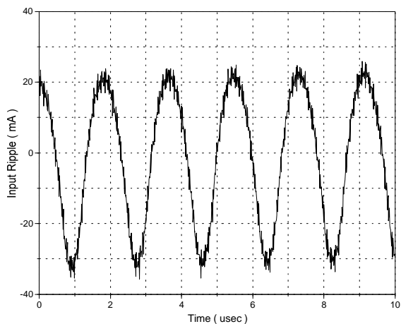
Input Ripple Current
