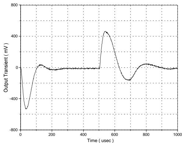
Output Load Transient Response 10% Load to/from 50% Load
