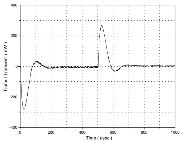
Output Load Transient Response 50% Load to/from 100% Load
