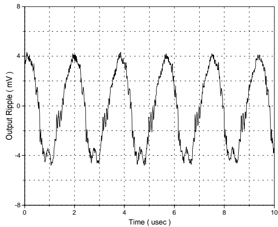
Output Ripple Voltage
