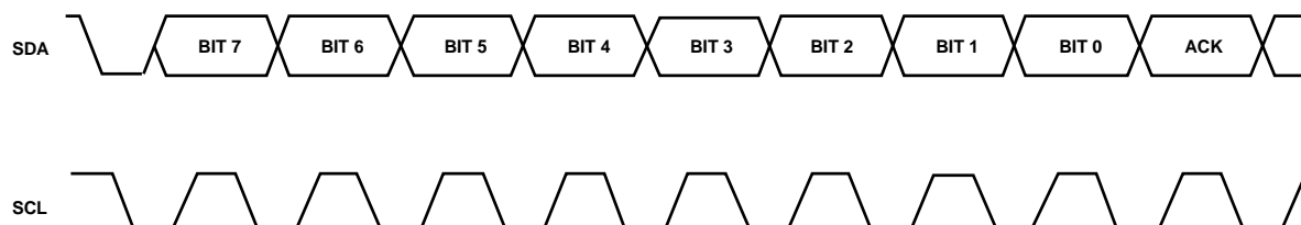
Figure 2. Serial Interface—Typical Byte Transfer
