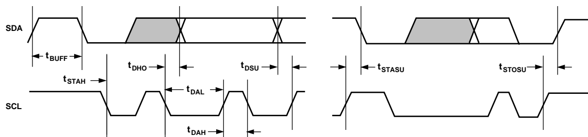
Figure 1. Serial Port Read/Write Timing
