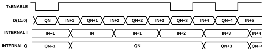
Figure 27. Continuous Mode Input Timing—TxENABLE Static High
