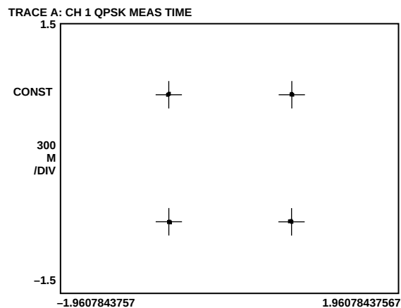
Figure 13. QPSK, 65 MHz, 2.56 MS/s
