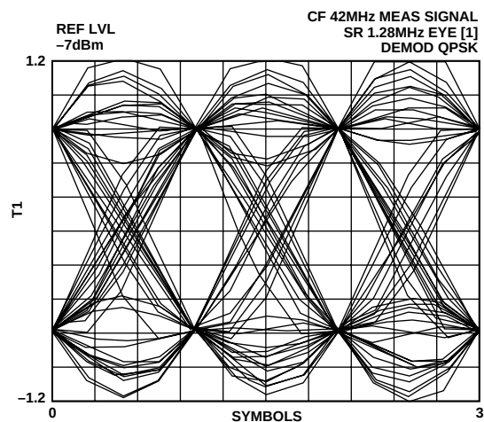
Figure 16. QPSK Modulation
