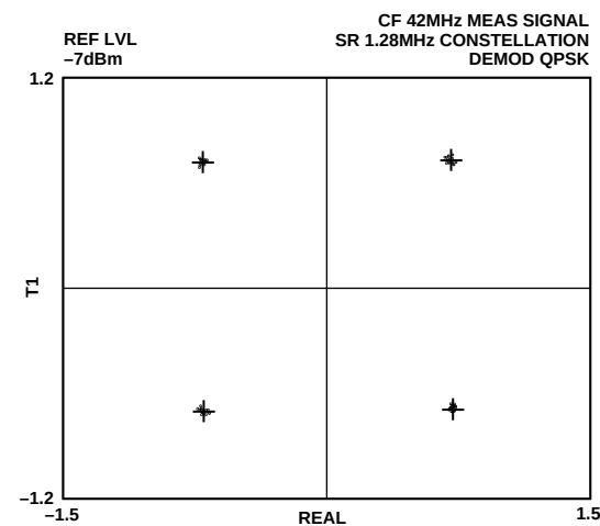
Figure 17. QPSK Modulation
