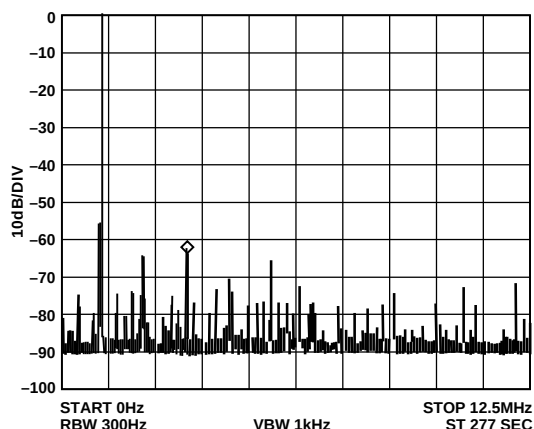
Figure 12. f_{MCLK} = 25 MHz, f_{OUT} = 1.1 MHz, Frequency Word = B439581
