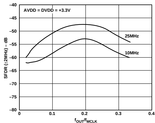
Figure 8. Wide Band SFDR vs. f_{\text{OUT}}/f_{\text{MCLK}} for Various MCLK Frequencies
