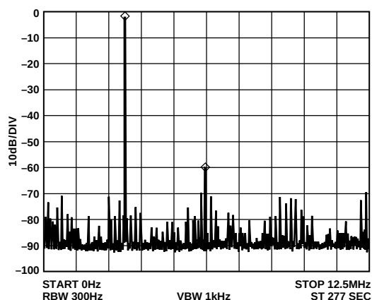
Figure 14. f_{MCLK} = 25 MHz, f_{OUT} = 3.1 MHz, Frequency Word = 1FBE76C9
