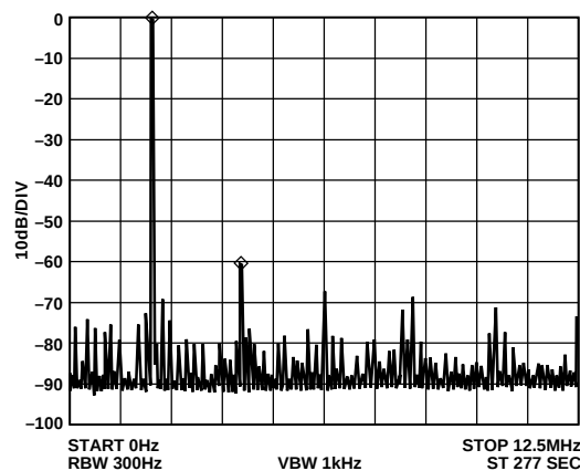
Figure 13. f_{MCLK} = 25 MHz, f_{OUT} = 2.1 MHz, Frequency Word = 15810625
