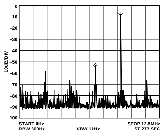
Figure 20. f_{MCLK} = 25 MHz, f_{OUT} = 9.1 MHz, Frequency Word = 5D2F1AA0
