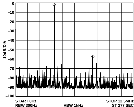
Figure 15. f_{MCLK} = 25 MHz, f_{OUT} = 4.1 MHz, Frequency Word = 29FBE76D
