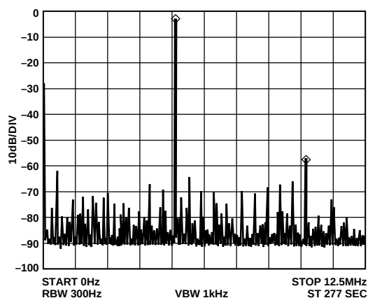
Figure 16. f_{MCLK} = 25 MHz, f_{OUT} = 5.1 MHz, Frequency Word = 34395810
