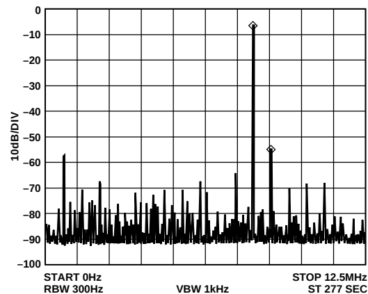
Figure 19. f_{MCLK} = 25 MHz, f_{OUT} = 8.1 MHz, Frequency Word = 52F1A9FC
