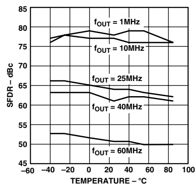
Figure 15. SFDR vs. Temperature @ 125 MSPS, 0 dBFS
