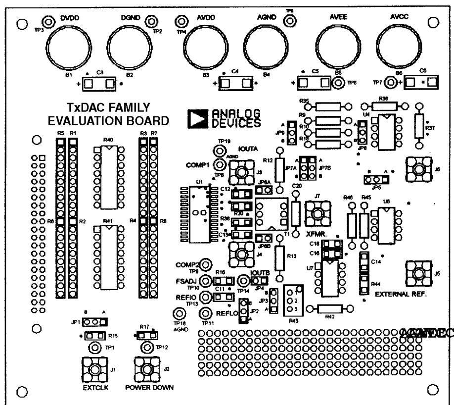
Figure 60. Silkscreen Layer—Top
