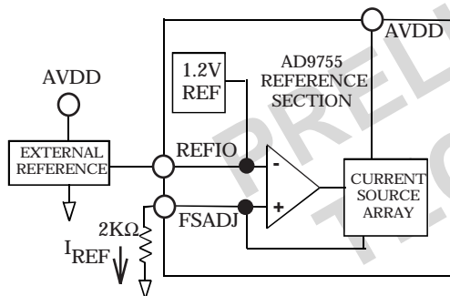
Figure 4. External Reference Configuration
