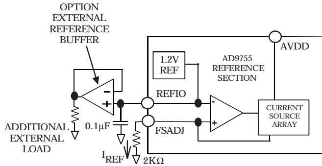
Figure 3. Internal Reference Configuration
