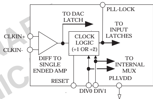
Figure 8. AD9755 Clock Circuitry with PLL Disabled
