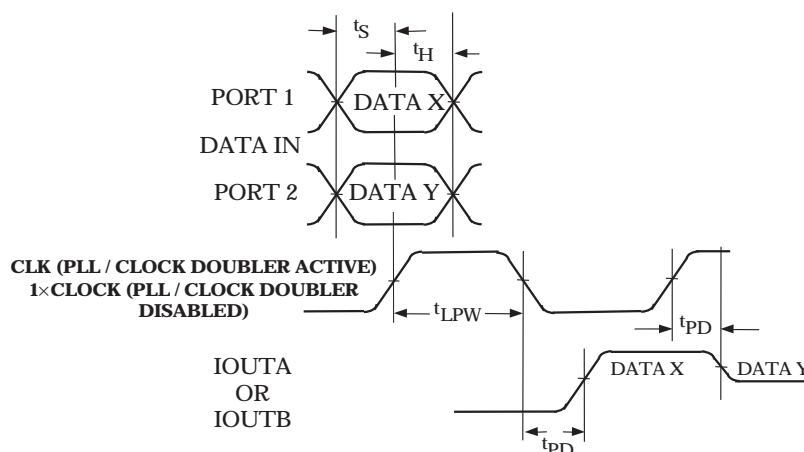
Figure 1. AD9755 I/O Timing
