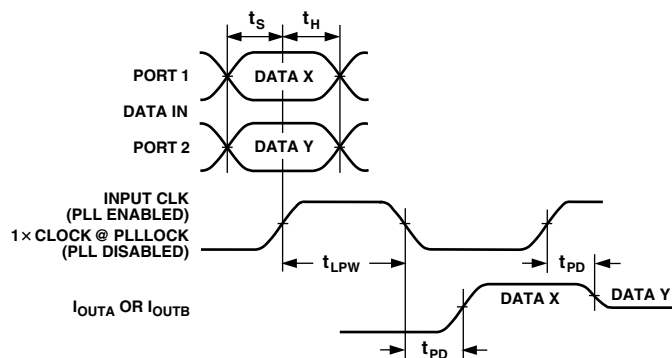
Figure 1. I/O Timing
