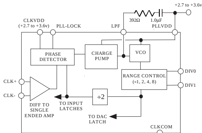
Figure 5. AD9751 Clock Circuitry with PLL Active
