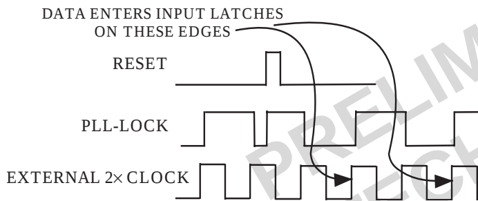
Figure 10. AD9751 Reset Function Timing with PLL Disabled
