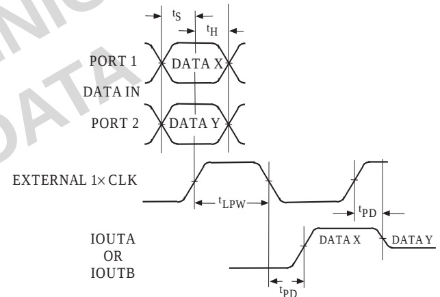
Figure 12. AD9751 Timing Requirements, Interleaved Mode with PLL Disabled, Clock Doubler Active
