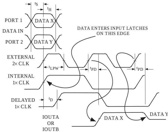
Figure 9. AD9751 Timing Requirements, Interleaved (2×) Mode with PLL Disabled
