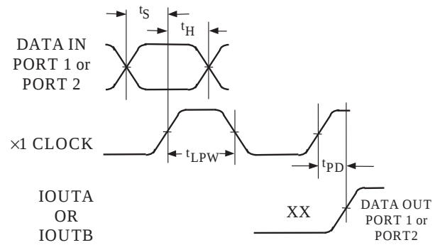
Figure 11. AD9751 Timing Requirements, Non-Interleaved Mode with PLL Disabled
