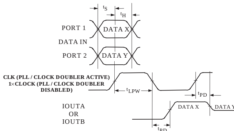
Figure 1. AD9751 I/O Timing
