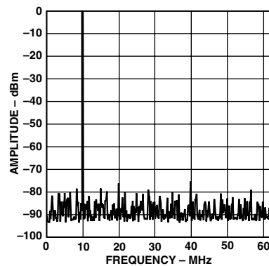
Figure 17. Single-Tone SFDR @ f_{CLK} = 125 \text{ MSPS}
