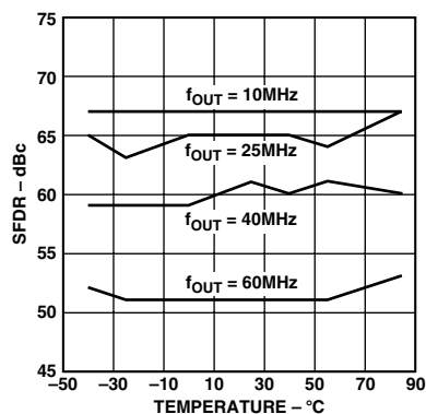
Figure 15. SFDR vs. Temperature @ f_{CLK} = 125 \text{ MSPS} , 0 \text{ dBFS}
