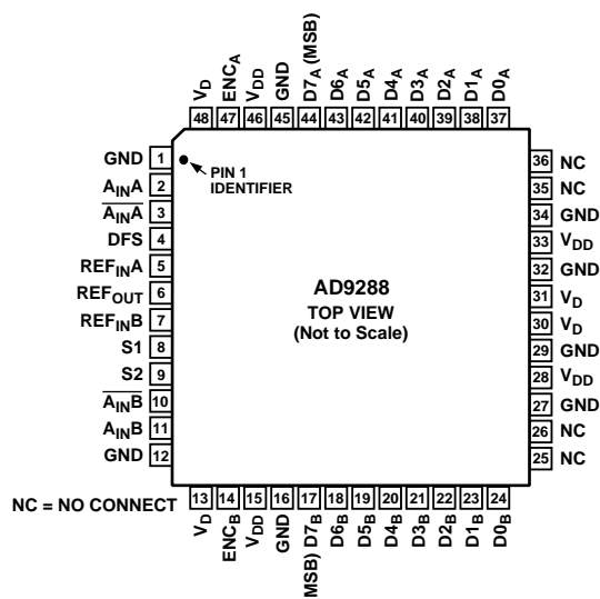
PIN FUNCTION DESCRIPTIONS
