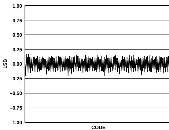
Figure 18. Differential Nonlinearity
