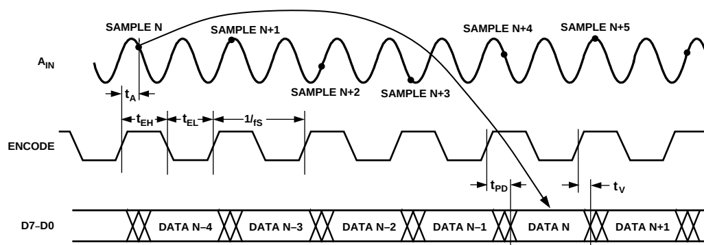
Figure 1. Timing Diagram
