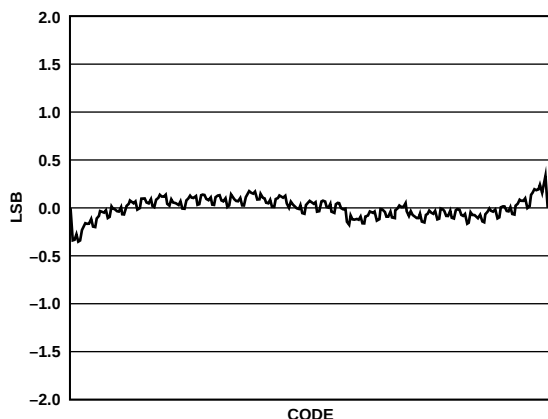
Figure 19. Integral Nonlinearity
