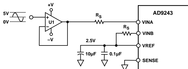
Figure 32. Single-Ended AD9243 Op Amp Drive Circuit
