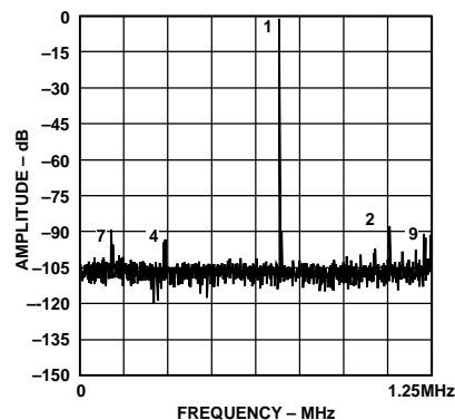
Figure 49. IF Sampling a 10.7 MHz Input Using the AD9243 ( V_{CM} = 2.5 \text{ V} , Input Span = 2 V p-p)
