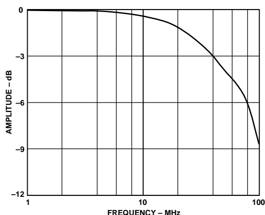
Figure 22. Full-Power Bandwidth
