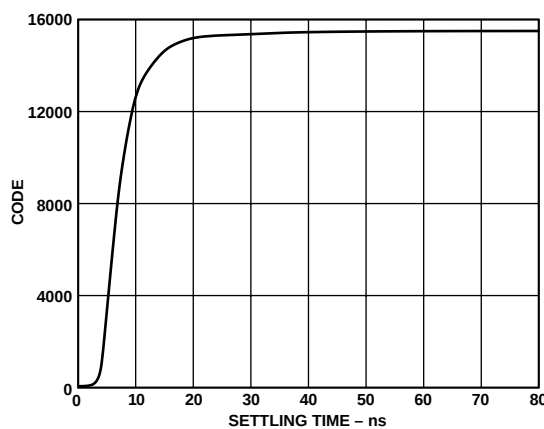
Figure 26. Settling Time
