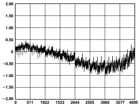
Figure 5. Typical INL
