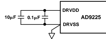
Figure 43. Digital Supply Decoupling
