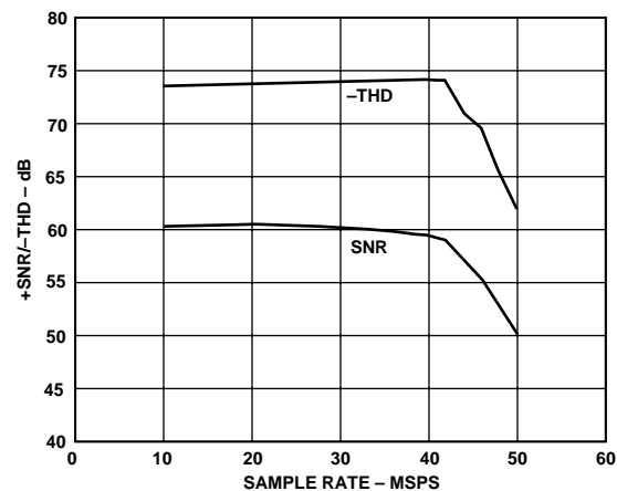
Figure 9. SNR and THD vs. Sample Rate ( f_{IN} = 20 MHz)
