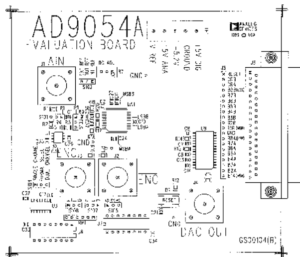
Figure 39. Assembly—Top View
