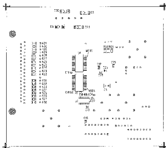
Figure 40. Assembly—Bottom View
