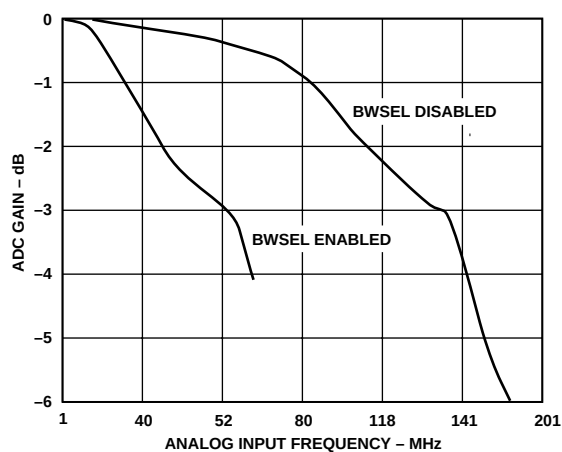
Figure 6. ADC Gain vs. AIN Frequency
