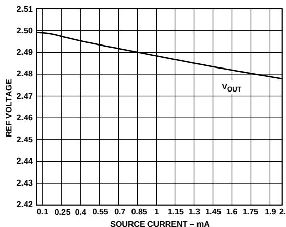
Figure 19. Reference Load Regulation
