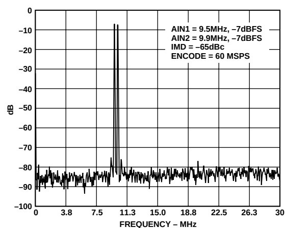
Figure 14. Two-Tone IMD
