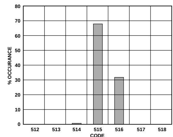
Figure 20. Midscale Histogram (Inputs Tied)
