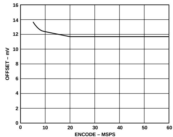
Figure 16. Offset vs. Clock Rate
