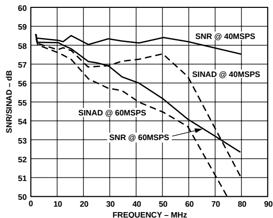
Figure 4. SNR/SINAD vs. AIN Frequency
