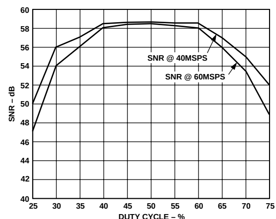
Figure 17. SNR vs. Duty Cycle
