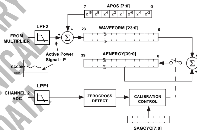
Figure 36 – AD7756 Energy Calibration
