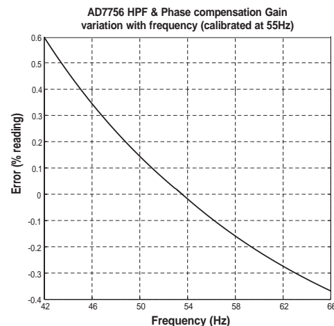
Figure 27c – Gain response of HPF & Phase Compensation (deviation of Gain as % of Gain at 54Hz)
