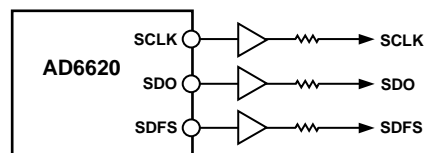
Figure 54. Serial Line Buffering and Series Source Termination
