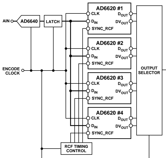
Figure 61. Parallel Processing with the AD6620
