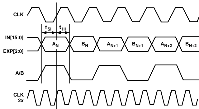
Figure 30. Full Rate Input Timing, Diversity Channel Real Mode
