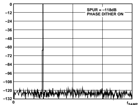
Figure 23. Typical NCO Spur with Dither
