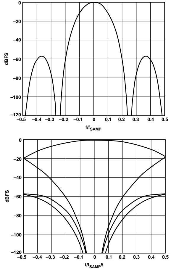
Figure 43. CIC5 Alias Rejection, M_{\text{CIC}5} = 4
