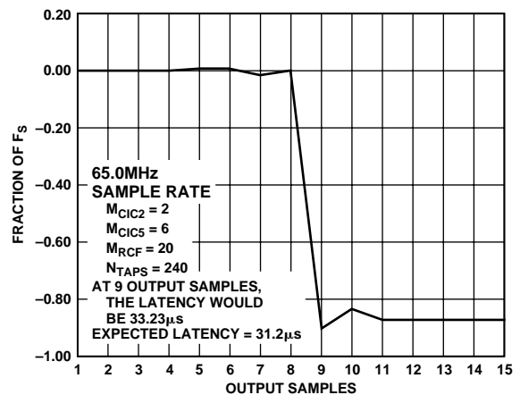
Figure 60. WB-GSM Example
