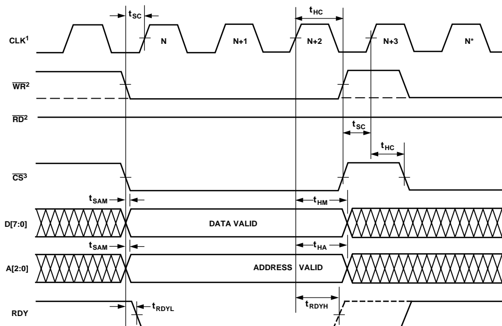
Figure 48. Mode 0 Read (MODE = GND)
