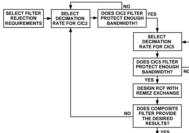
Figure 53. Diagram of Filter Design Software
