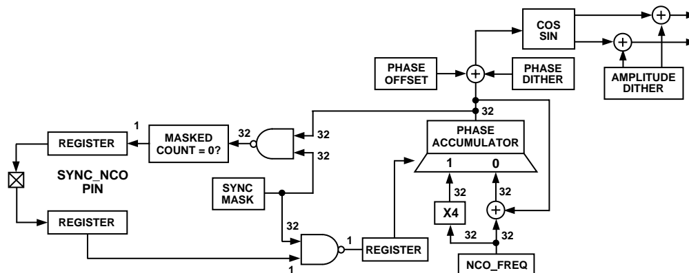
Figure 40. NCO Block Diagram
