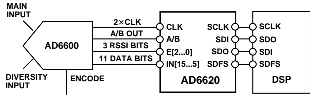
Figure 65. Implementation of a Narrow Band Receiver
