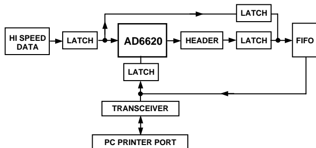
Figure 52. Evaluation Board Block Diagram
