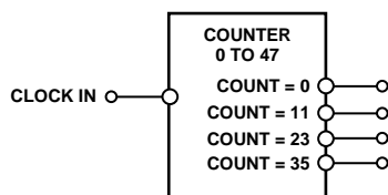
Figure 62. RCF Timing Generator for Parallel Processing
