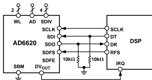
Figure 56. AD6620 Configured as a Serial Slave
