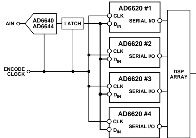
Figure 66. Implementation of a Multicarrier Receiver
