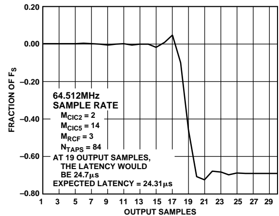
Figure 59. PHS Example
