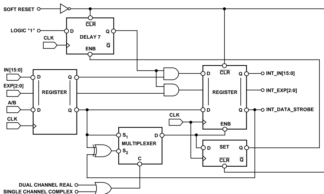
Figure 32. Simplified Input Data Port Schematic for the AD6620
