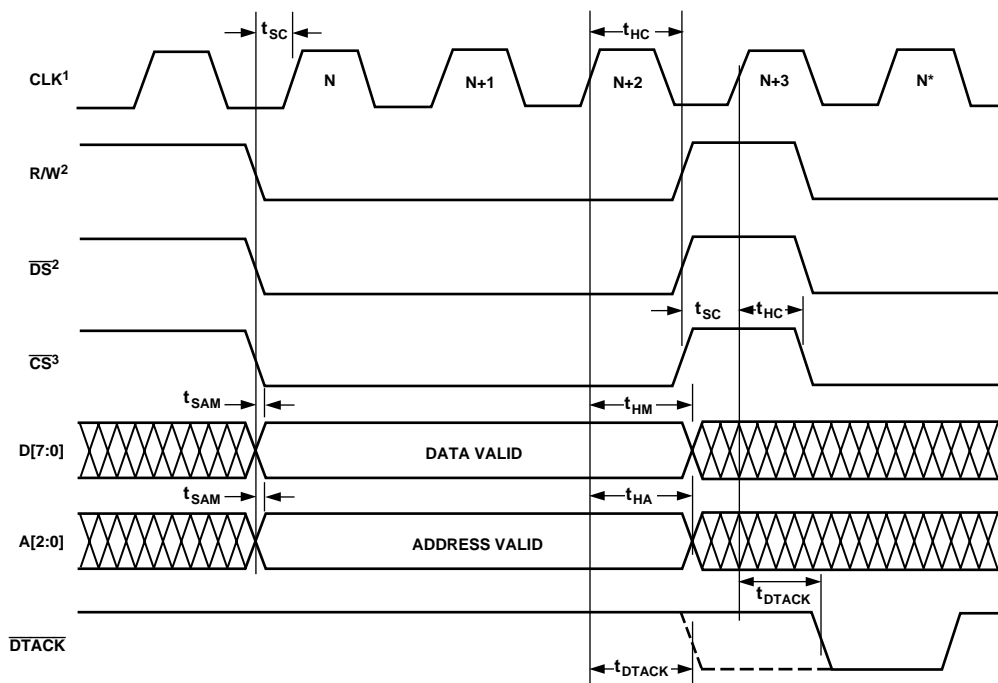
Figure 50. Mode 1 Read (MODE = VDD)
