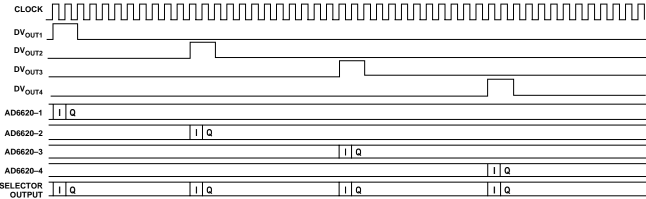
Figure 64. Timing for Parallel Processing
