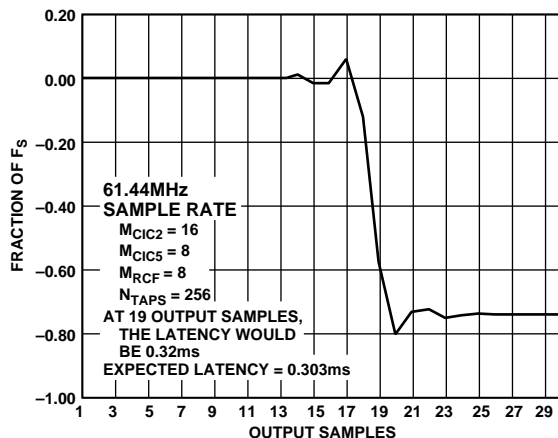
Figure 57. AMPS Example
