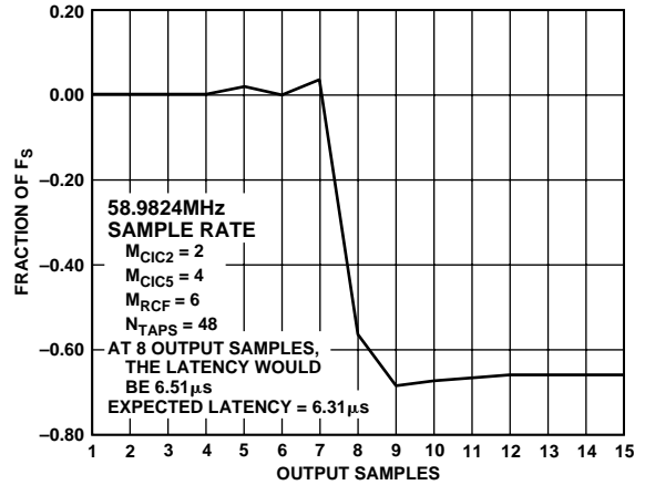
Figure 58. CDMA Example
