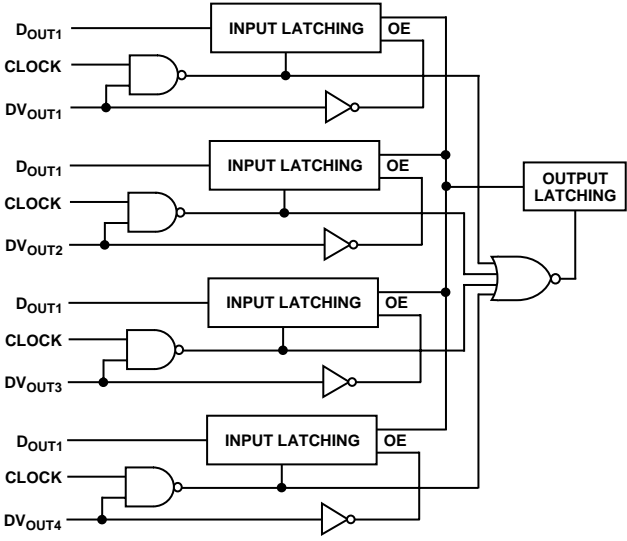
Figure 63. Parallel Processing Output Selector
