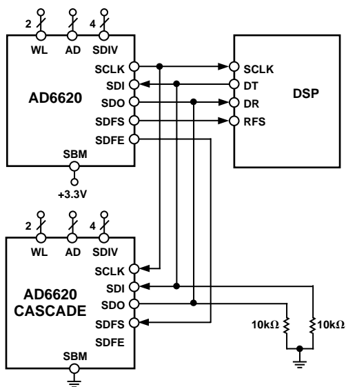
Figure 55. Dual AD6620s Using the Serial Bus in a TDM Application
