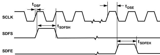
Figure 11. Serial Frame Switching Characteristics
