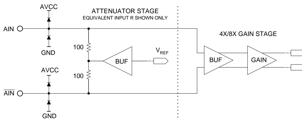
Figure 2. Analog Input Stage (Channel A shown; Channel B is equivalent)
