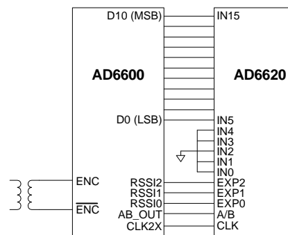
Figure 31. AD6600/AD6620 Connections
