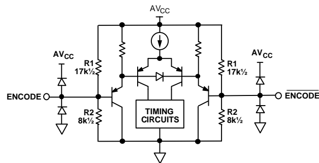
Figure 5. Encode Inputs
